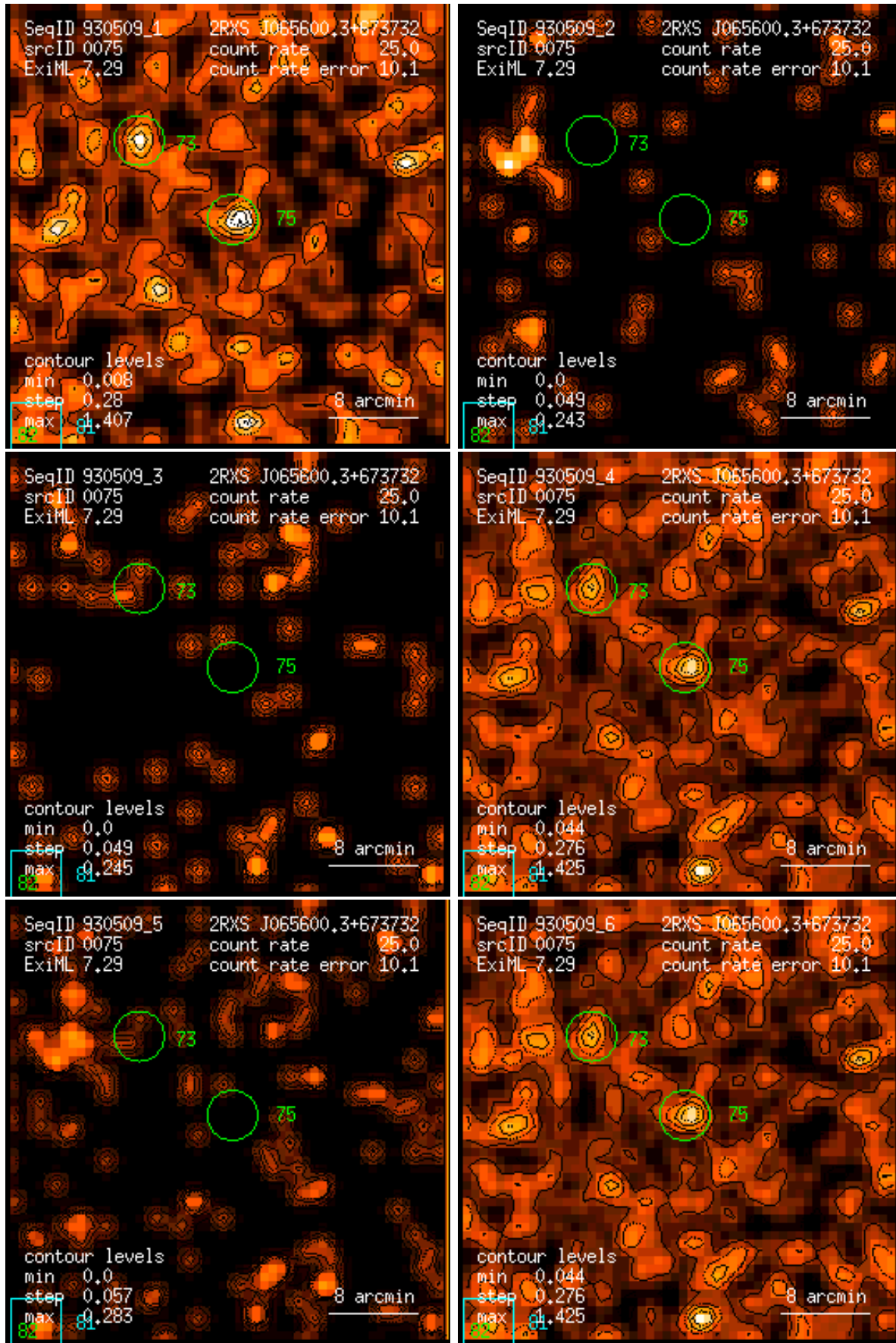
Figure 75: RASS 930509: detection 0075: band rate images, Gaussian filter: (1) PSPC channels 11 – 41, (2) 52 – 90, (3) 91 – 201, (4) 11 – 235, (5) 52 – 201, (6) 11 – 201. Broad band rates in counts/ks. Band rate contour levels in counts/ks/arcmin 2 .
