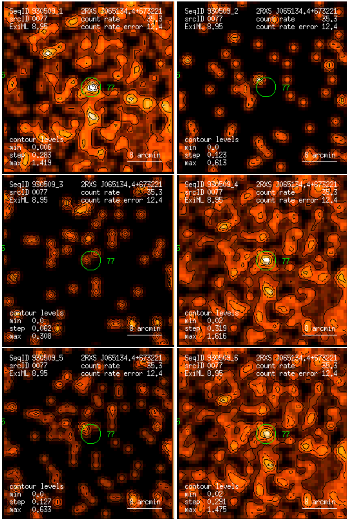
Figure 77: RASS 930509: detection 0077: band rate images, Gaussian filter: (1) PSPC channels 11 – 41, (2) 52 – 90, (3) 91 – 201, (4) 11 – 235, (5) 52 – 201, (6) 11 – 201. Broad band rates in counts/ks. Band rate contour levels in counts/ks/arcmin 2 .
