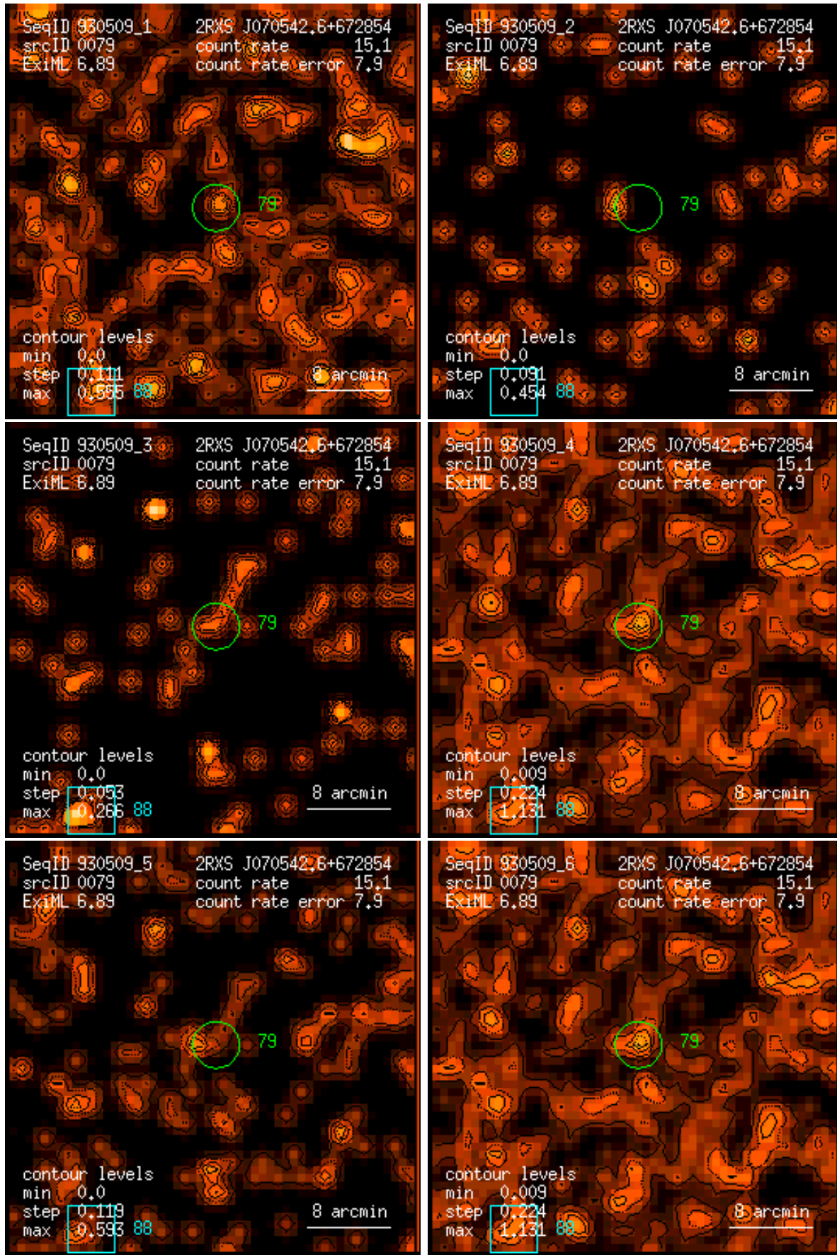
Figure 79: RASS 930509: detection 0079: band rate images, Gaussian filter: (1) PSPC channels 11 – 41, (2) 52 – 90, (3) 91 – 201, (4) 11 – 235, (5) 52 – 201, (6) 11 – 201. Broad band rates in counts/ks. Band rate contour levels in counts/ks/arcmin 2 .
