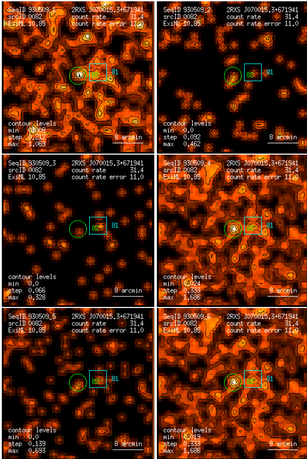
Figure 82: RASS 930509: detection 0082: band rate images, Gaussian filter: (1) PSPC channels 11 – 41, (2) 52 – 90, (3) 91 – 201, (4) 11 – 235, (5) 52 – 201, (6) 11 – 201. Broad band rates in counts/ks. Band rate contour levels in counts/ks/arcmin 2 .
