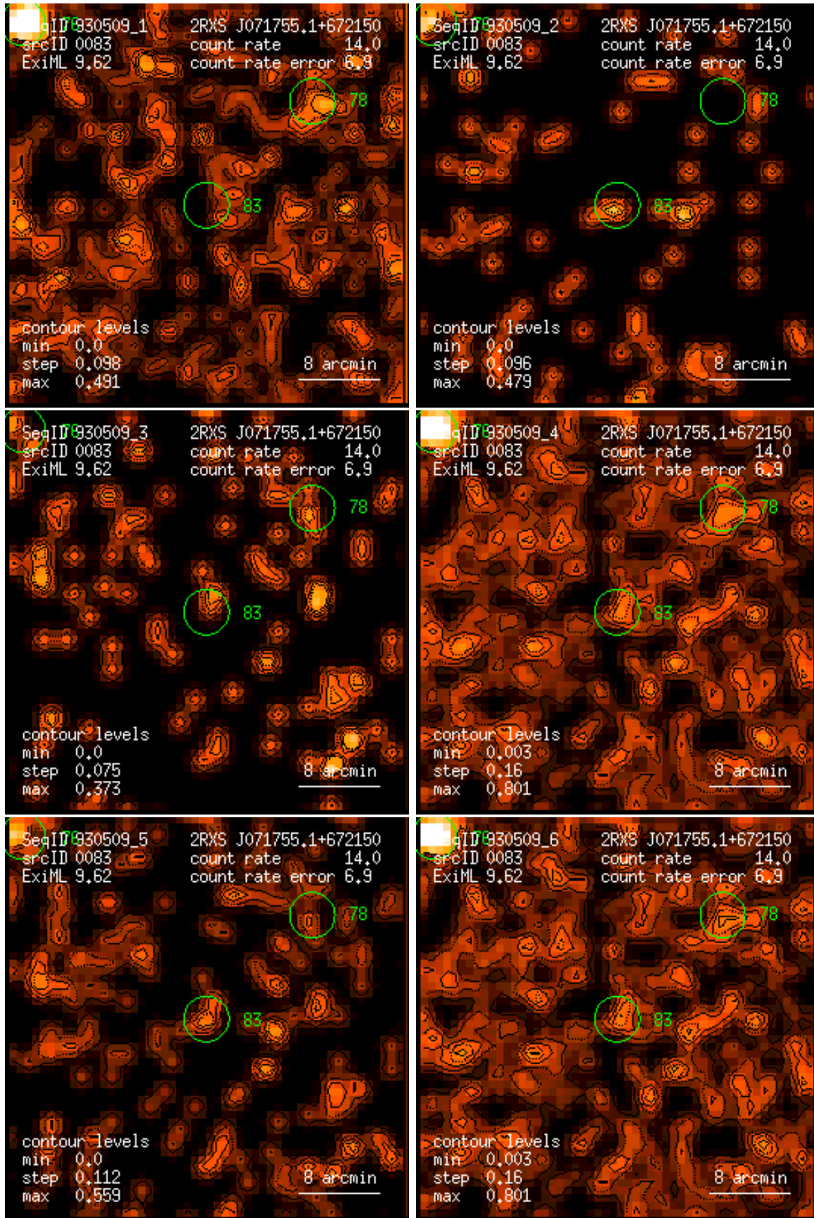
Figure 83: RASS 930509: detection 0083: band rate images, Gaussian filter: (1) PSPC channels 11 – 41, (2) 52 – 90, (3) 91 – 201, (4) 11 – 235, (5) 52 – 201, (6) 11 – 201. Broad band rates in counts/ks. Band rate contour levels in counts/ks/arcmin 2 .
