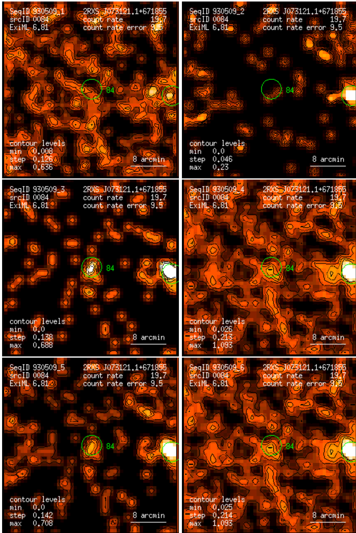
Figure 84: RASS 930509: detection 0084: band rate images, Gaussian filter: (1) PSPC channels 11 – 41, (2) 52 – 90, (3) 91 – 201, (4) 11 – 235, (5) 52 – 201, (6) 11 – 201. Broad band rates in counts/ks. Band rate contour levels in counts/ks/arcmin 2 .
