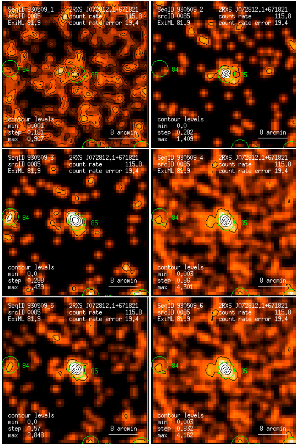
Figure 85: RASS 930509: detection 0085: band rate images, Gaussian filter: (1) PSPC channels 11 – 41, (2) 52 – 90, (3) 91 – 201, (4) 11 – 235, (5) 52 – 201, (6) 11 – 201. Broad band rates in counts/ks. Band rate contour levels in counts/ks/arcmin 2 .
