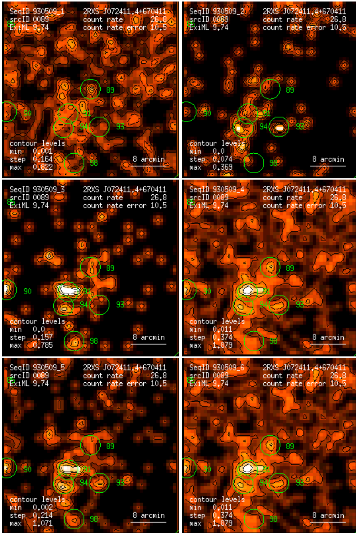
Figure 89: RASS 930509: detection 0089: band rate images, Gaussian filter: (1) PSPC channels 11 – 41, (2) 52 – 90, (3) 91 – 201, (4) 11 – 235, (5) 52 – 201, (6) 11 – 201. Broad band rates in counts/ks. Band rate contour levels in counts/ks/arcmin 2 .
