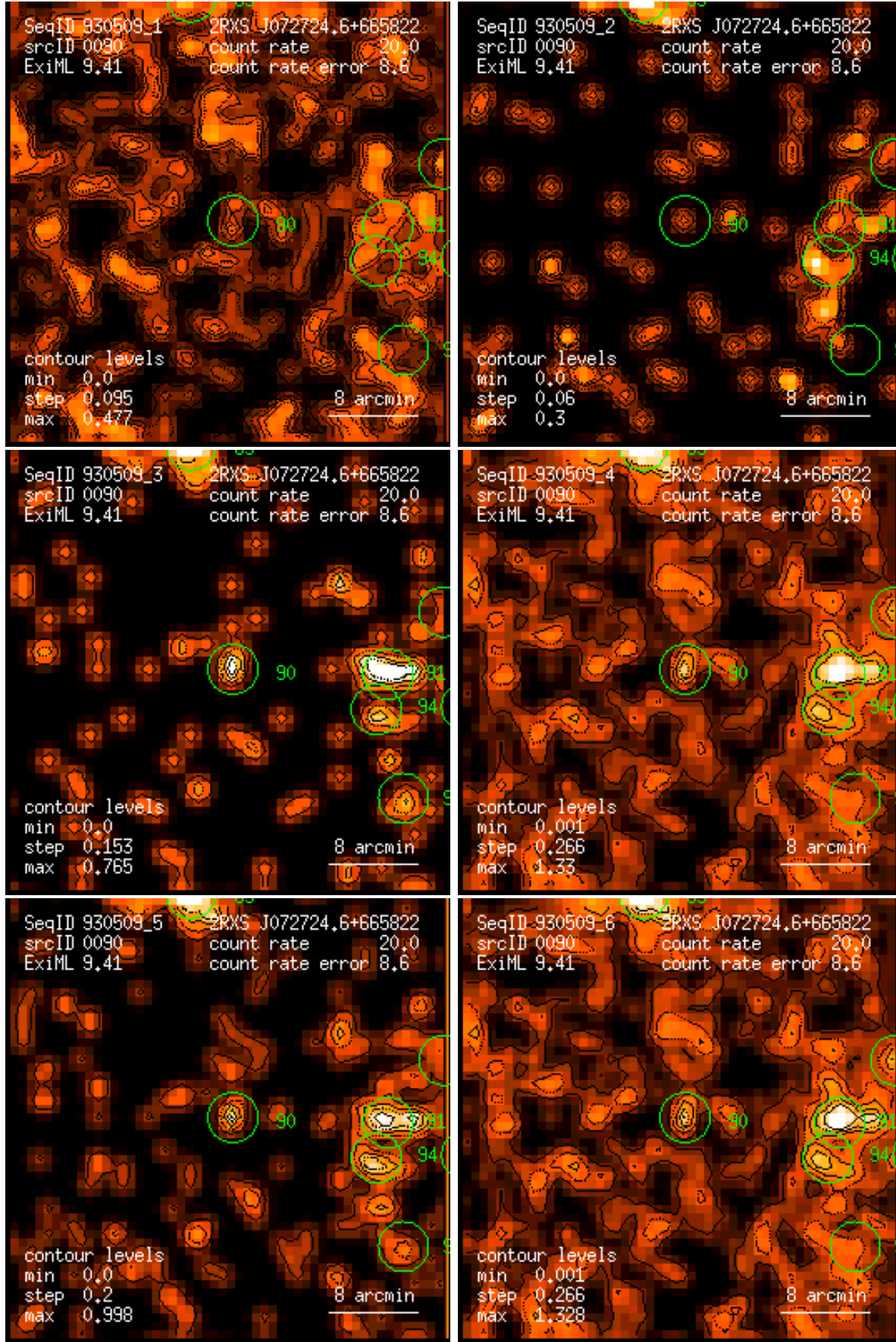
Figure 90: RASS 930509: detection 0090: band rate images, Gaussian filter: (1) PSPC channels 11 – 41, (2) 52 – 90, (3) 91 – 201, (4) 11 – 235, (5) 52 – 201, (6) 11 – 201. Broad band rates in counts/ks. Band rate contour levels in counts/ks/arcmin 2 .
