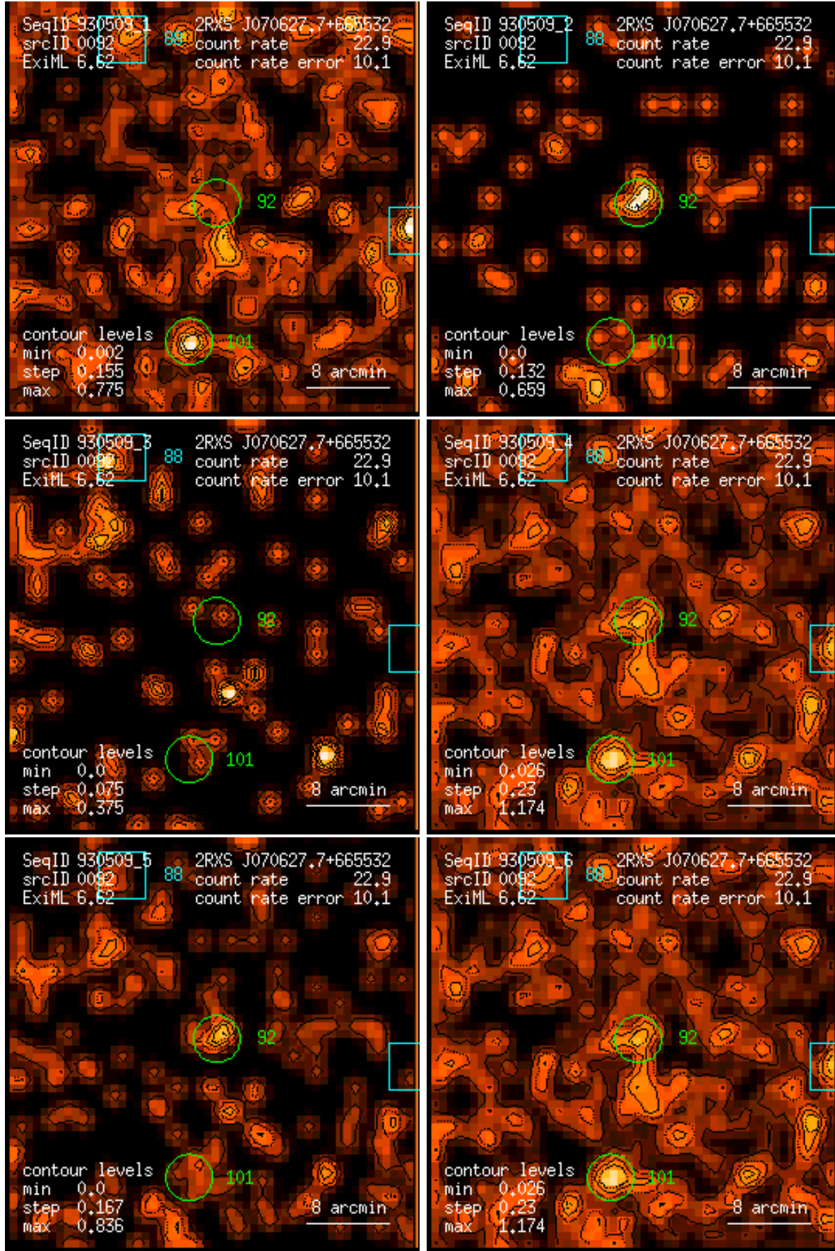
Figure 92: RASS 930509: detection 0092: band rate images, Gaussian filter: (1) PSPC channels 11 – 41, (2) 52 – 90, (3) 91 – 201, (4) 11 – 235, (5) 52 – 201, (6) 11 – 201. Broad band rates in counts/ks. Band rate contour levels in counts/ks/arcmin 2 .
