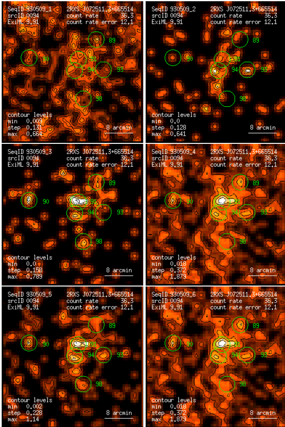
Figure 94: RASS 930509: detection 0094: band rate images, Gaussian filter: (1) PSPC channels 11 – 41, (2) 52 – 90, (3) 91 – 201, (4) 11 – 235, (5) 52 – 201, (6) 11 – 201. Broad band rates in counts/ks. Band rate contour levels in counts/ks/arcmin 2 .
