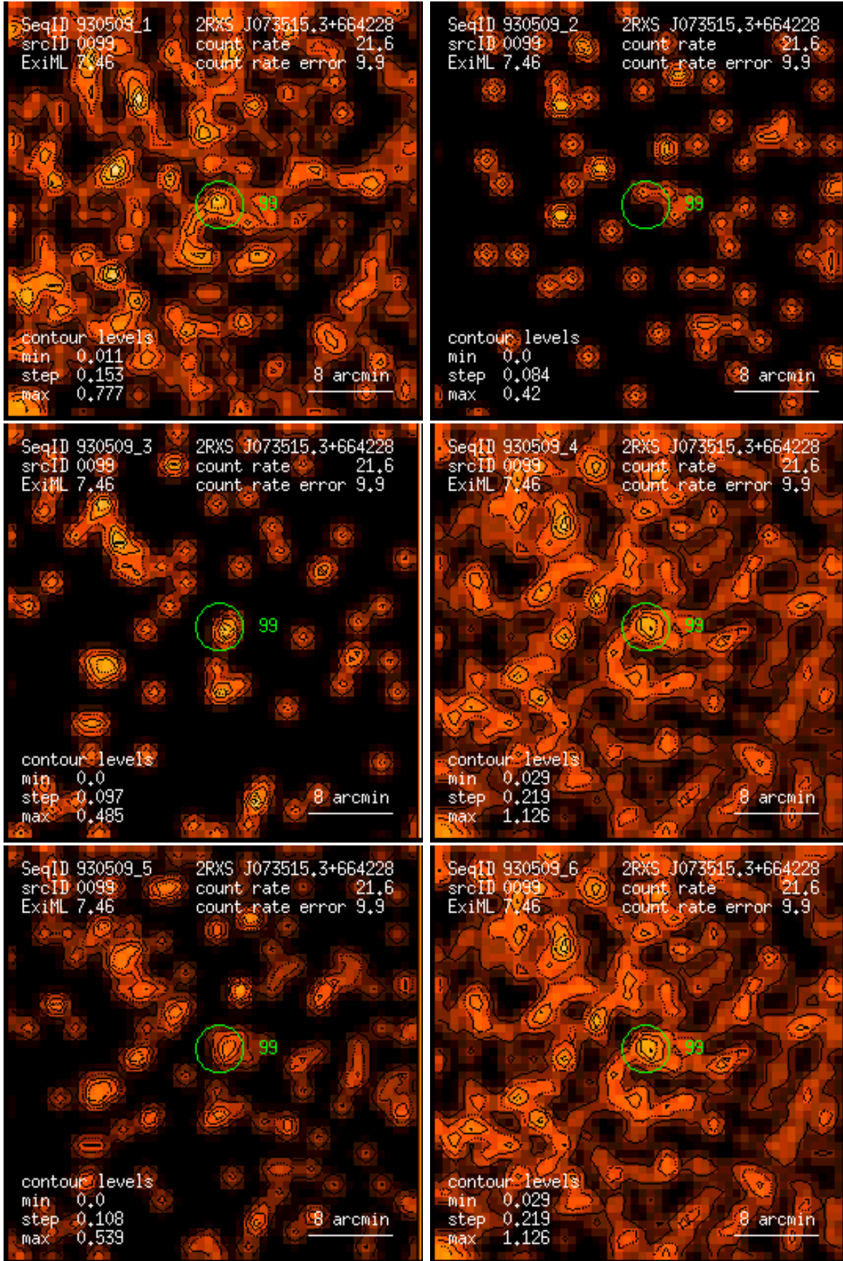
Figure 99: RASS 930509: detection 0099: band rate images, Gaussian filter: (1) PSPC channels 11 – 41, (2) 52 – 90, (3) 91 – 201, (4) 11 – 235, (5) 52 – 201, (6) 11 – 201. Broad band rates in counts/ks. Band rate contour levels in counts/ks/arcmin 2 .
