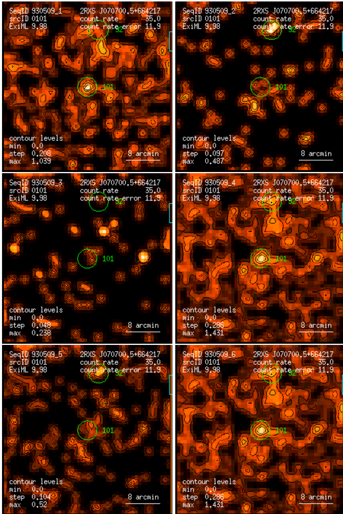
Figure 101: RASS 930509: detection 0101: band rate images, Gaussian filter: (1) PSPC channels 11 – 41, (2) 52 – 90, (3) 91 – 201, (4) 11 – 235, (5) 52 – 201, (6) 11 – 201. Broad band rates in counts/ks. Band rate contour levels in counts/ks/arcmin 2 .
