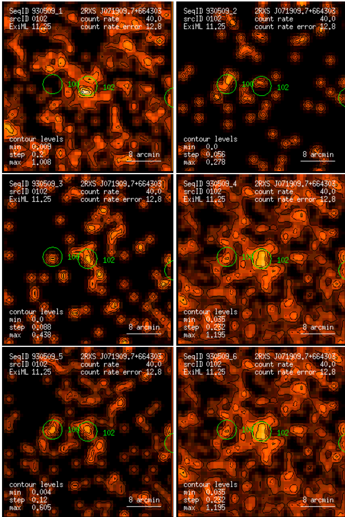
Figure 102: RASS 930509: detection 0102: band rate images, Gaussian filter: (1) PSPC channels 11 – 41, (2) 52 – 90, (3) 91 – 201, (4) 11 – 235, (5) 52 – 201, (6) 11 – 201. Broad band rates in counts/ks. Band rate contour levels in counts/ks/arcmin 2 .
