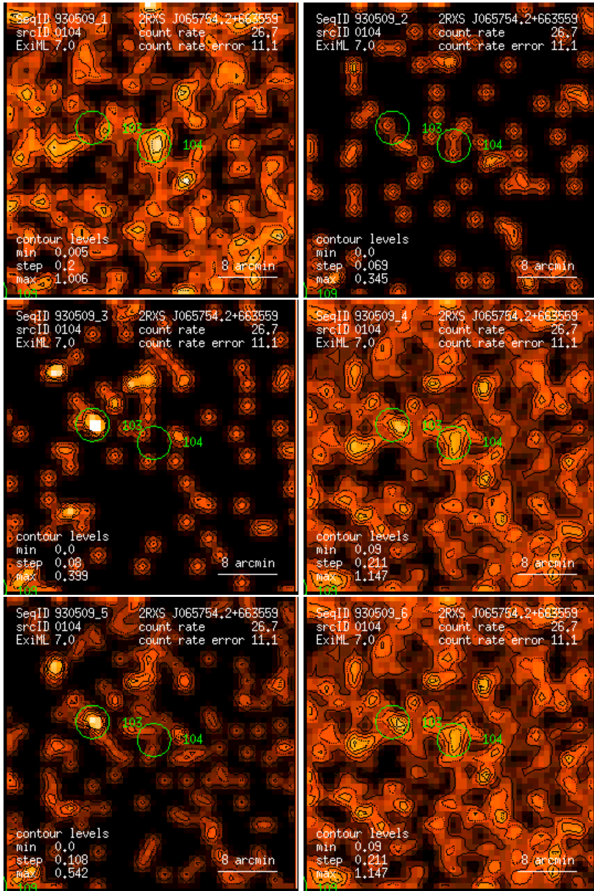
Figure 104: RASS 930509: detection 0104: band rate images, Gaussian filter: (1) PSPC channels 11 – 41, (2) 52 – 90, (3) 91 – 201, (4) 11 – 235, (5) 52 – 201, (6) 11 – 201. Broad band rates in counts/ks. Band rate contour levels in counts/ks/arcmin 2 .
