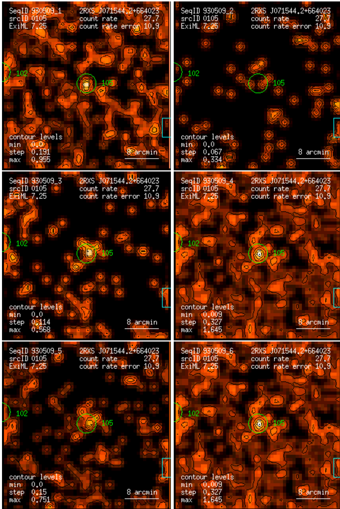
Figure 105: RASS 930509: detection 0105: band rate images, Gaussian filter: (1) PSPC channels 11 – 41, (2) 52 – 90, (3) 91 – 201, (4) 11 – 235, (5) 52 – 201, (6) 11 – 201. Broad band rates in counts/ks. Band rate contour levels in counts/ks/arcmin 2 .
