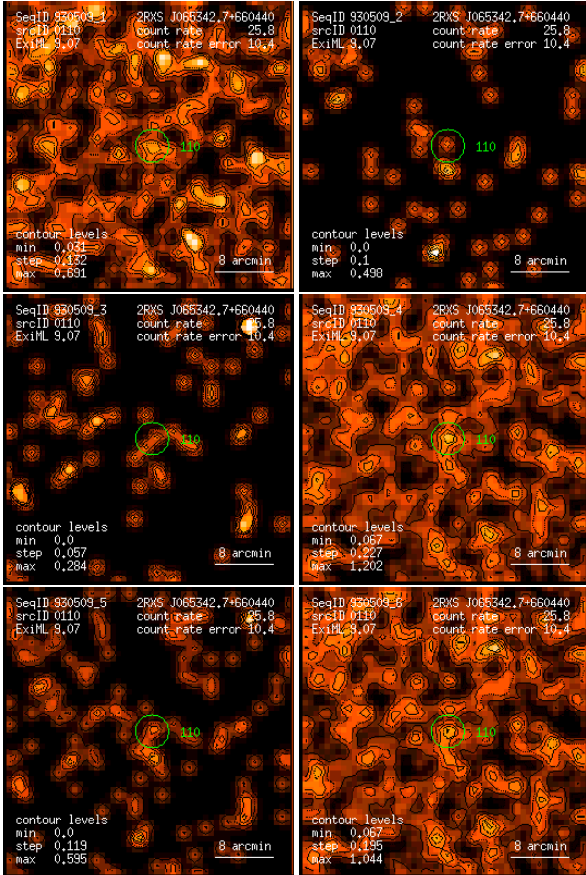
Figure 110: RASS 930509: detection 0110: band rate images, Gaussian filter: (1) PSPC channels 11 – 41, (2) 52 – 90, (3) 91 – 201, (4) 11 – 235, (5) 52 – 201, (6) 11 – 201. Broad band rates in counts/ks. Band rate contour levels in counts/ks/arcmin 2 .
