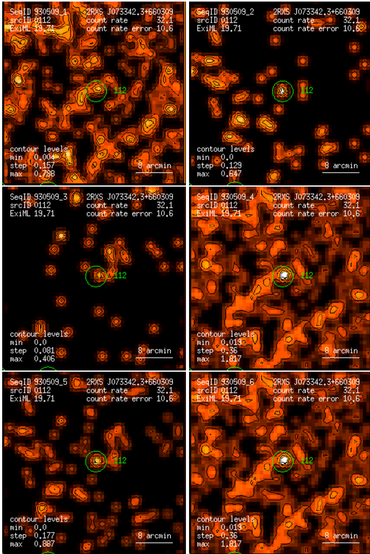
Figure 112: RASS 930509: detection 0112: band rate images, Gaussian filter: (1) PSPC channels 11 – 41, (2) 52 – 90, (3) 91 – 201, (4) 11 – 235, (5) 52 – 201, (6) 11 – 201. Broad band rates in counts/ks. Band rate contour levels in counts/ks/arcmin 2 .
