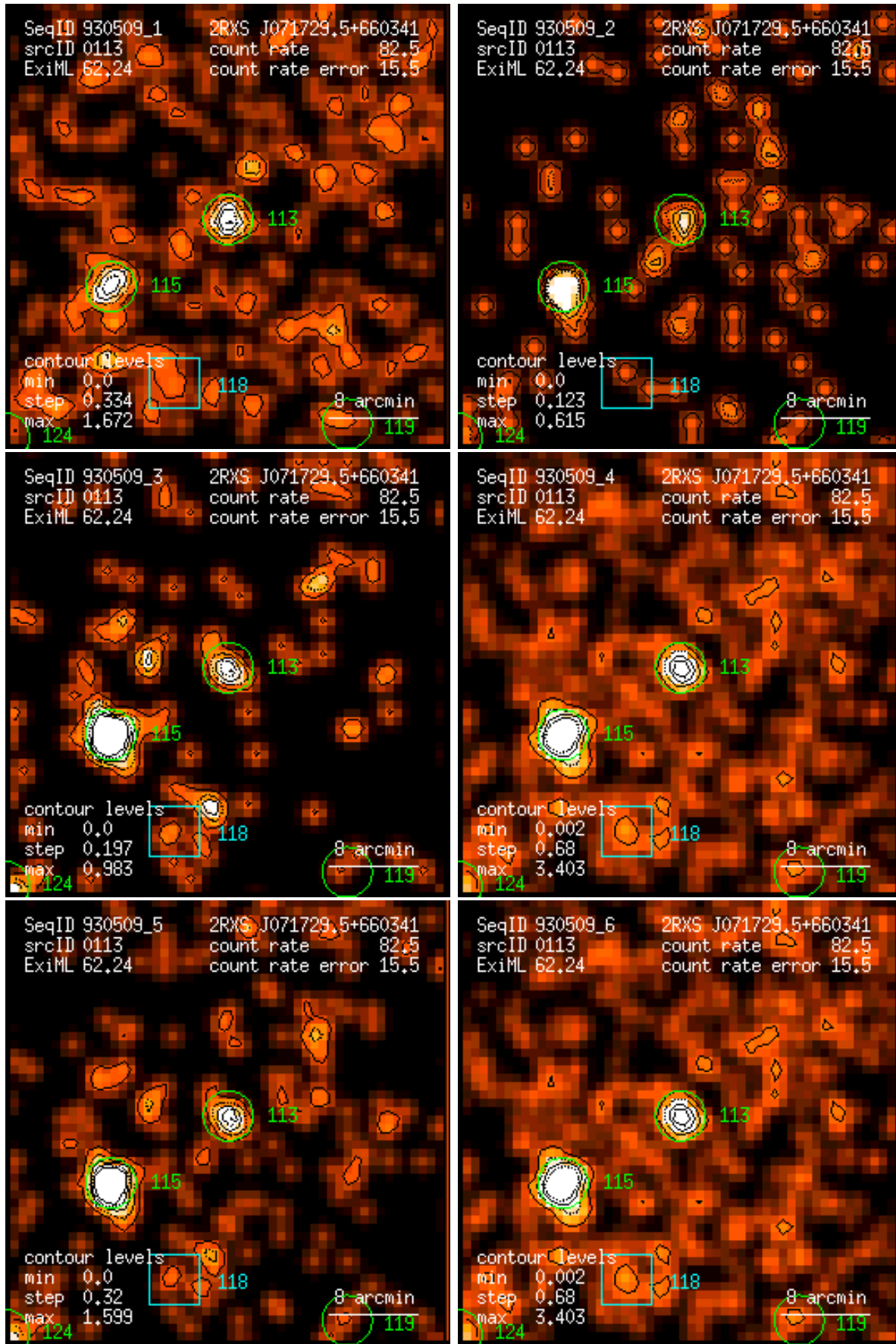
Figure 113: RASS 930509: detection 0113: band rate images, Gaussian filter: (1) PSPC channels 11 – 41, (2) 52 – 90, (3) 91 – 201, (4) 11 – 235, (5) 52 – 201, (6) 11 – 201. Broad band rates in counts/ks. Band rate contour levels in counts/ks/arcmin 2 .
