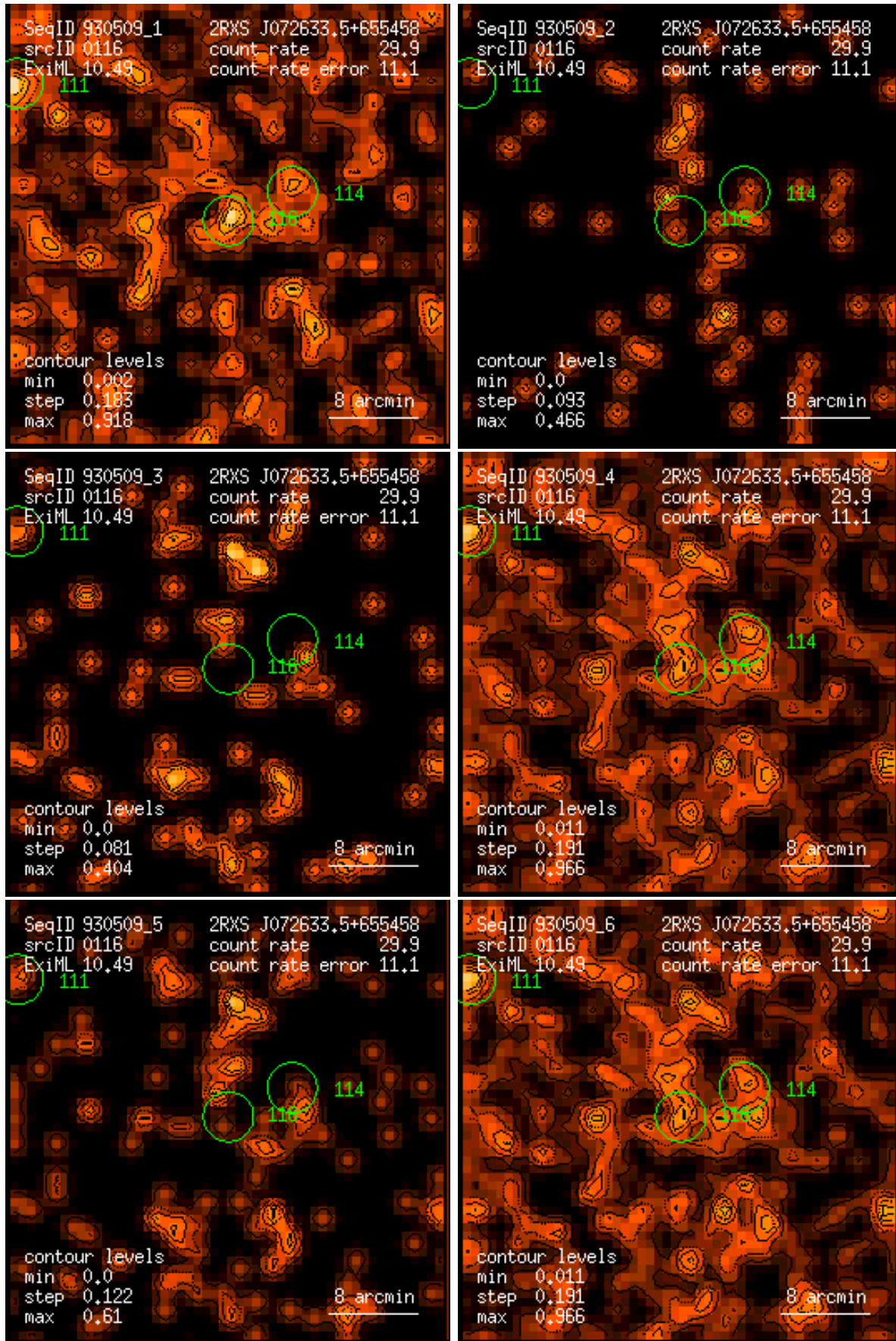
Figure 116: RASS 930509: detection 0116: band rate images, Gaussian filter: (1) PSPC channels 11 – 41, (2) 52 – 90, (3) 91 – 201, (4) 11 – 235, (5) 52 – 201, (6) 11 – 201. Broad band rates in counts/ks. Band rate contour levels in counts/ks/arcmin 2 .
