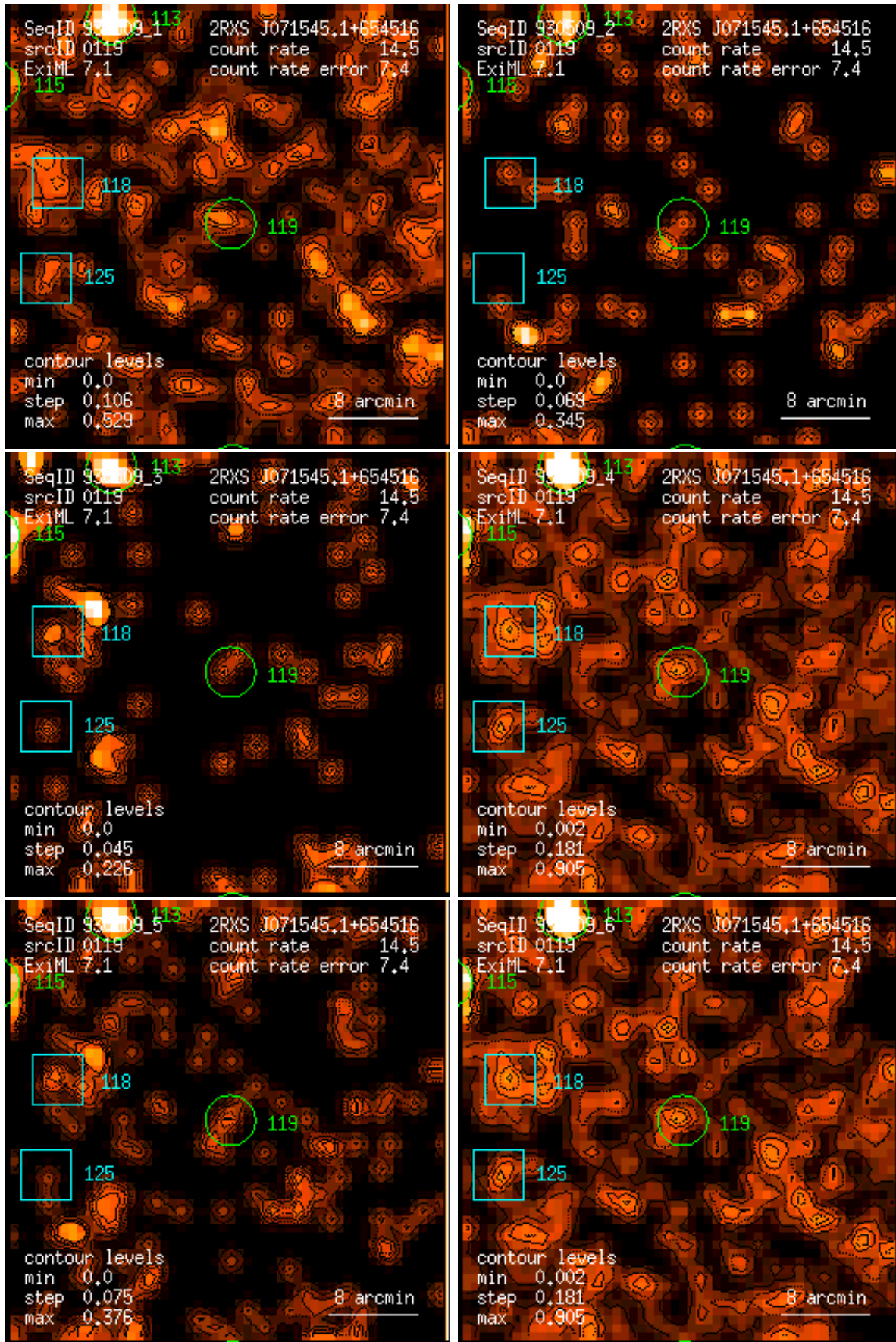
Figure 119: RASS 930509: detection 0119: band rate images, Gaussian filter: (1) PSPC channels 11 – 41, (2) 52 – 90, (3) 91 – 201, (4) 11 – 235, (5) 52 – 201, (6) 11 – 201. Broad band rates in counts/ks. Band rate contour levels in counts/ks/arcmin 2 .
