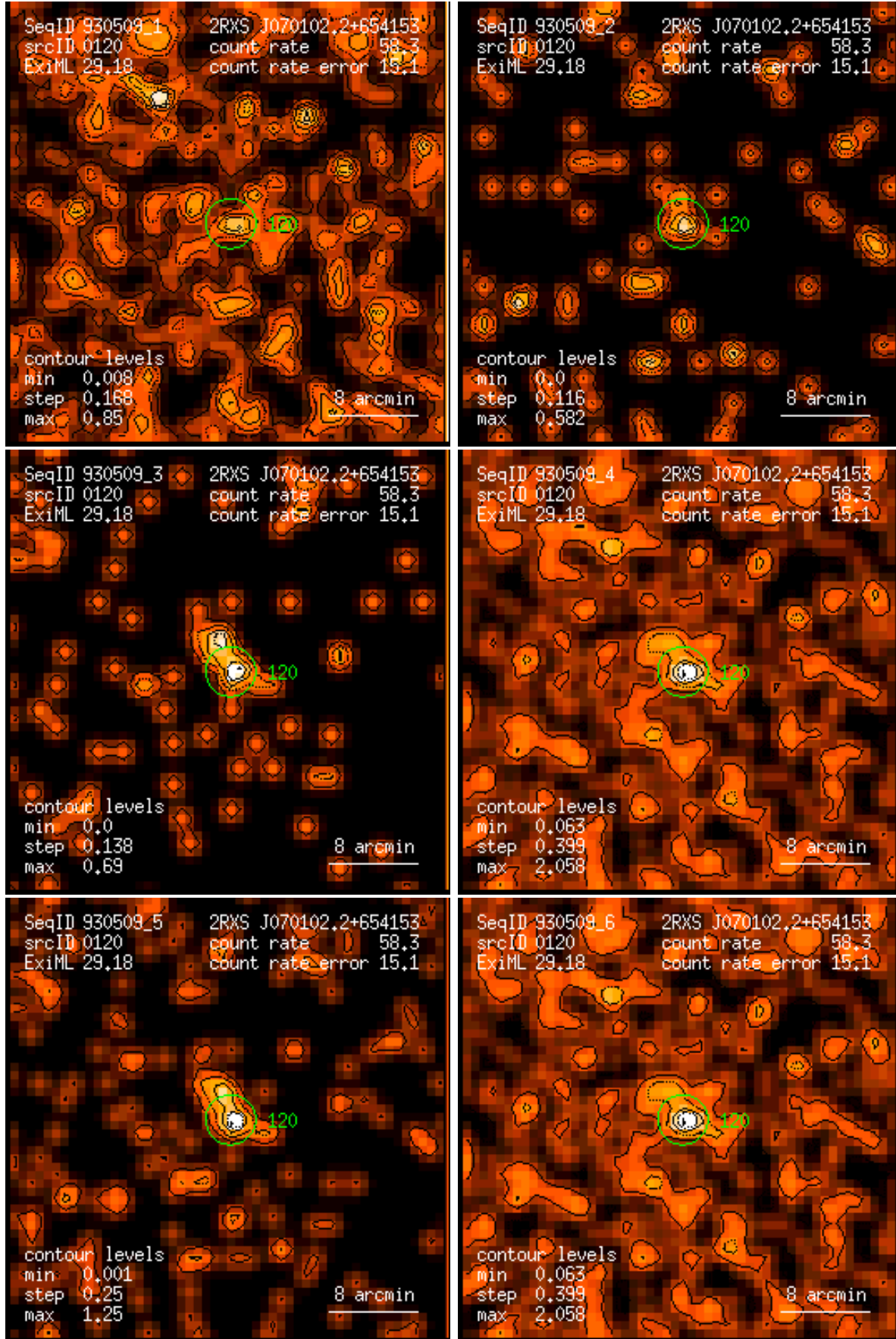
Figure 120: RASS 930509: detection 0120: band rate images, Gaussian filter: (1) PSPC channels 11 – 41, (2) 52 – 90, (3) 91 – 201, (4) 11 – 235, (5) 52 – 201, (6) 11 – 201. Broad band rates in counts/ks. Band rate contour levels in counts/ks/arcmin 2 .
