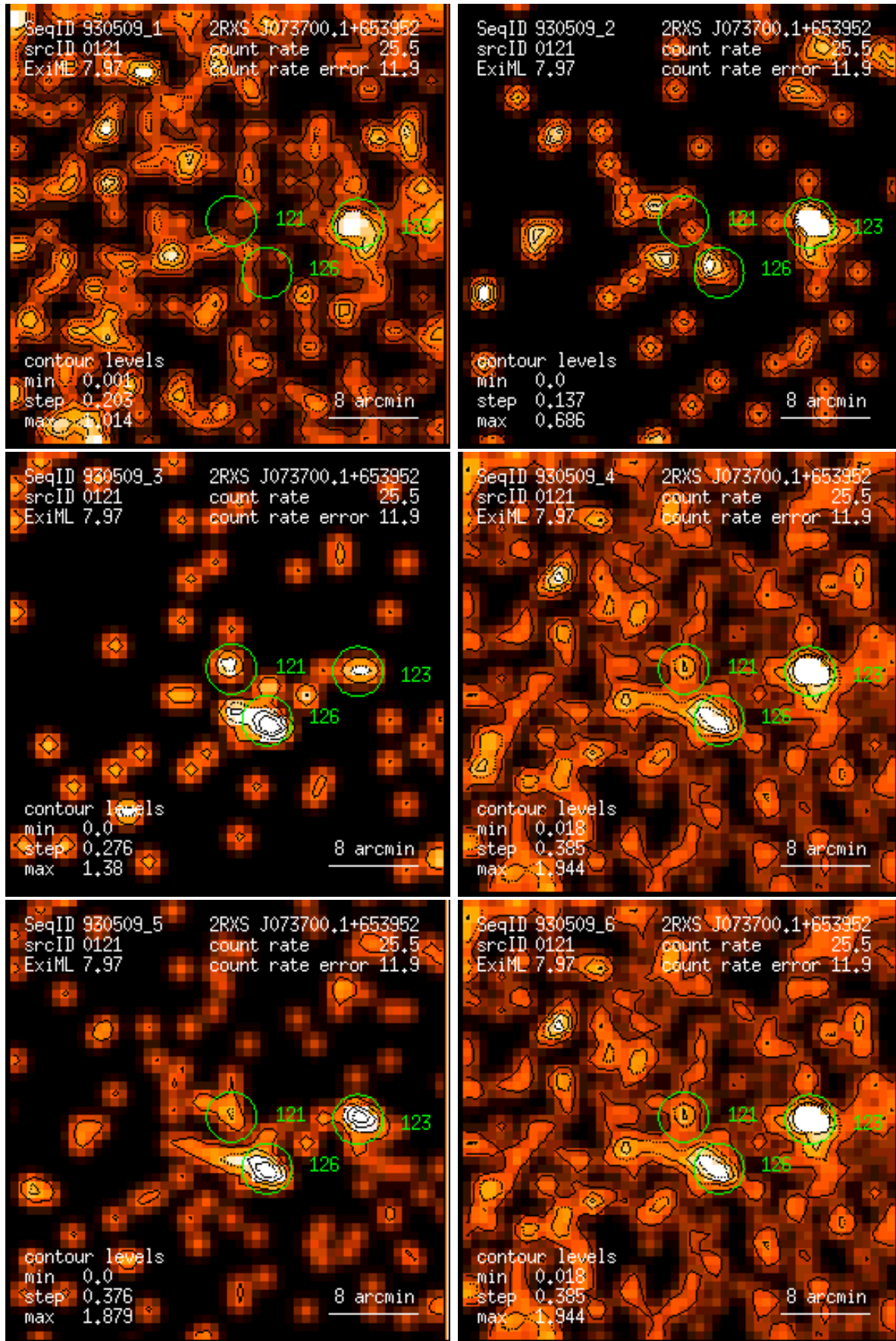
Figure 121: RASS 930509: detection 0121: band rate images, Gaussian filter: (1) PSPC channels 11 – 41, (2) 52 – 90, (3) 91 – 201, (4) 11 – 235, (5) 52 – 201, (6) 11 – 201. Broad band rates in counts/ks. Band rate contour levels in counts/ks/arcmin 2 .
