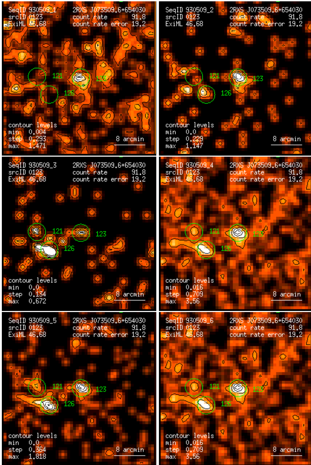
Figure 123: RASS 930509: detection 0123: band rate images, Gaussian filter: (1) PSPC channels 11 – 41, (2) 52 – 90, (3) 91 – 201, (4) 11 – 235, (5) 52 – 201, (6) 11 – 201. Broad band rates in counts/ks. Band rate contour levels in counts/ks/arcmin 2 .
