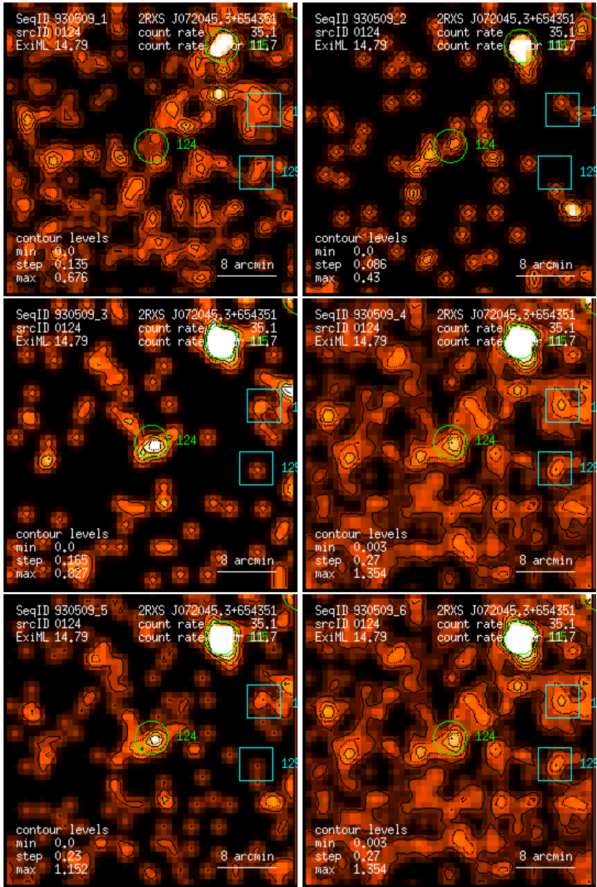
Figure 124: RASS 930509: detection 0124: band rate images, Gaussian filter: (1) PSPC channels 11 – 41, (2) 52 – 90, (3) 91 – 201, (4) 11 – 235, (5) 52 – 201, (6) 11 – 201. Broad band rates in counts/ks. Band rate contour levels in counts/ks/arcmin 2 .
