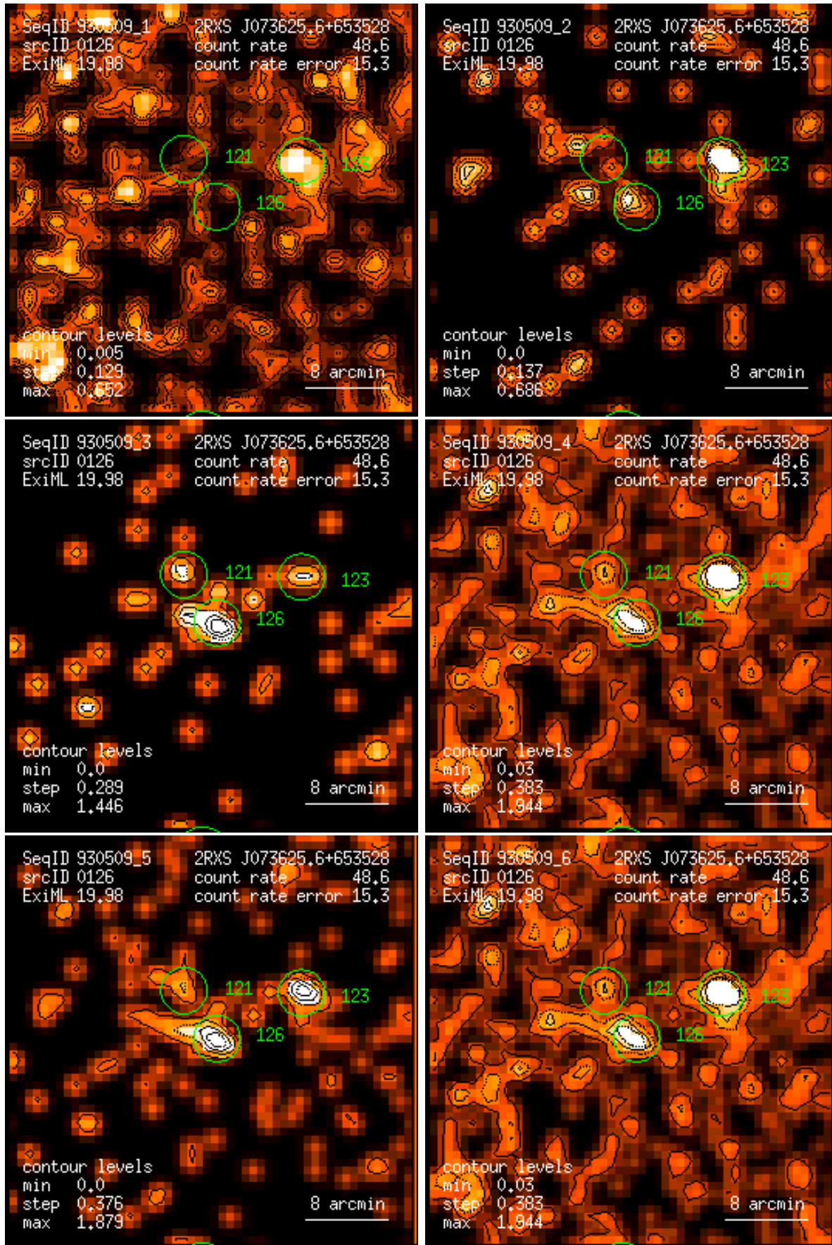
Figure 126: RASS 930509: detection 0126: band rate images, Gaussian filter: (1) PSPC channels 11 – 41, (2) 52 – 90, (3) 91 – 201, (4) 11 – 235, (5) 52 – 201, (6) 11 – 201. Broad band rates in counts/ks. Band rate contour levels in counts/ks/arcmin 2 .
