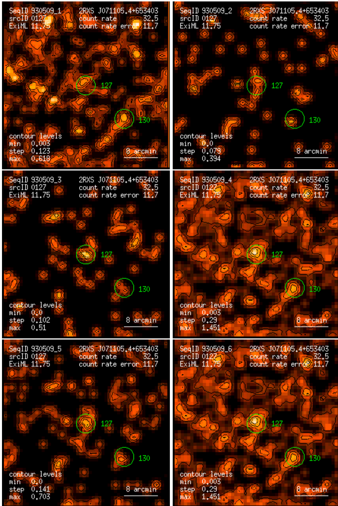
Figure 127: RASS 930509: detection 0127: band rate images, Gaussian filter: (1) PSPC channels 11 – 41, (2) 52 – 90, (3) 91 – 201, (4) 11 – 235, (5) 52 – 201, (6) 11 – 201. Broad band rates in counts/ks. Band rate contour levels in counts/ks/arcmin 2 .
