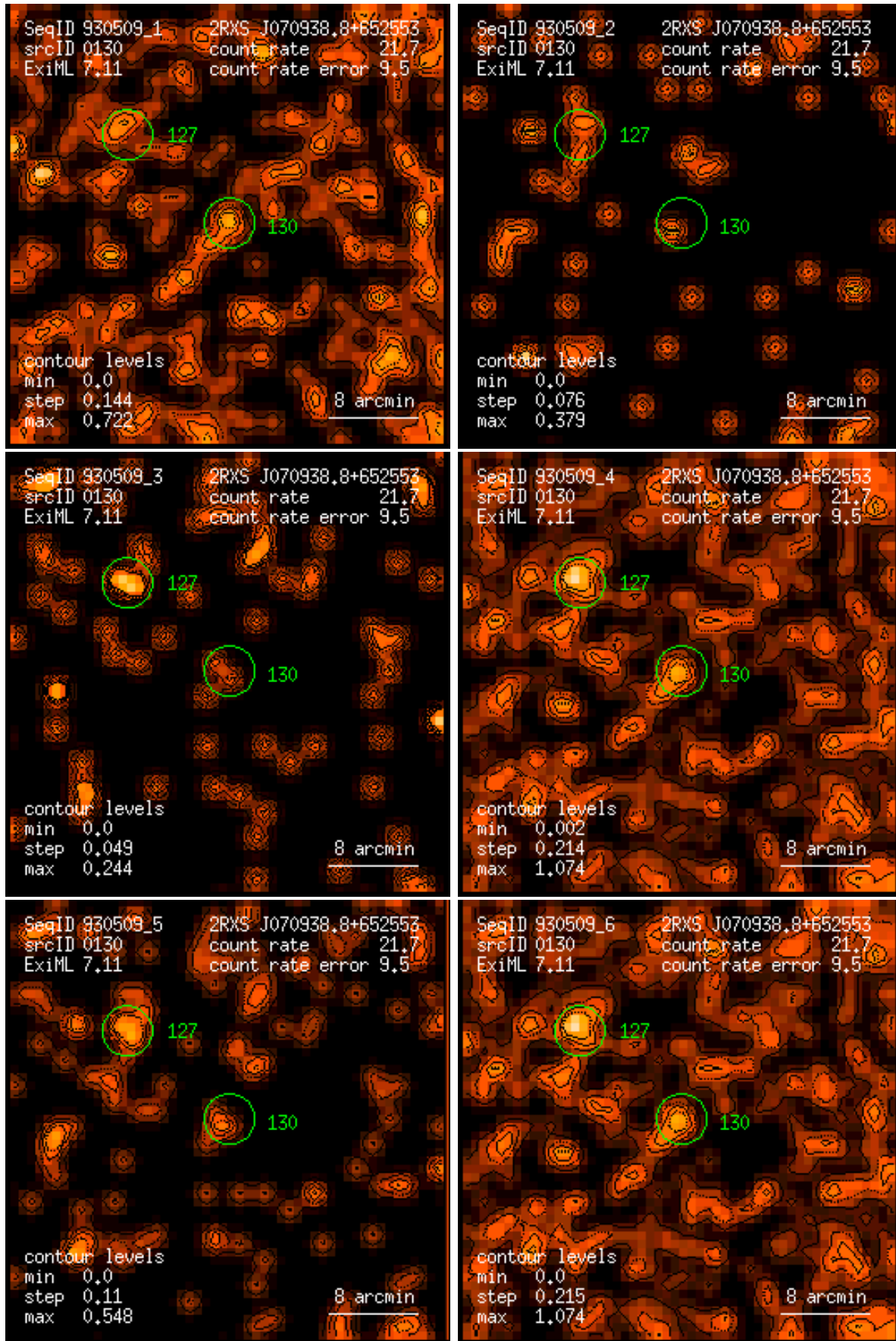
Figure 130: RASS 930509: detection 0130: band rate images, Gaussian filter: (1) PSPC channels 11 – 41, (2) 52 – 90, (3) 91 – 201, (4) 11 – 235, (5) 52 – 201, (6) 11 – 201. Broad band rates in counts/ks. Band rate contour levels in counts/ks/arcmin 2 .
