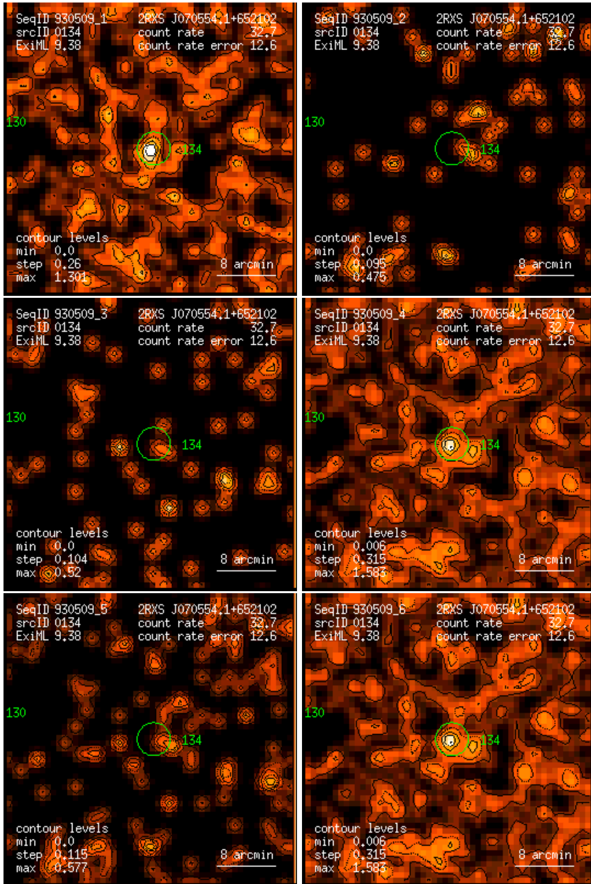
Figure 134: RASS 930509: detection 0134: band rate images, Gaussian filter: (1) PSPC channels 11 – 41, (2) 52 – 90, (3) 91 – 201, (4) 11 – 235, (5) 52 – 201, (6) 11 – 201. Broad band rates in counts/ks. Band rate contour levels in counts/ks/arcmin 2 .
