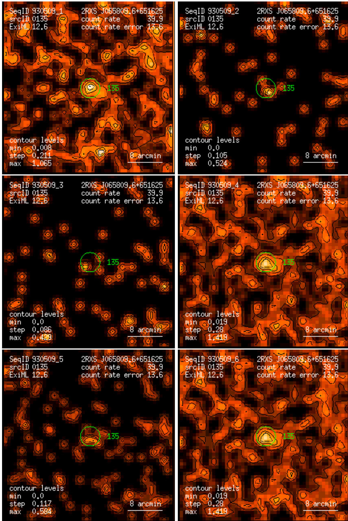
Figure 135: RASS 930509: detection 0135: band rate images, Gaussian filter: (1) PSPC channels 11 – 41, (2) 52 – 90, (3) 91 – 201, (4) 11 – 235, (5) 52 – 201, (6) 11 – 201. Broad band rates in counts/ks. Band rate contour levels in counts/ks/arcmin 2 .
