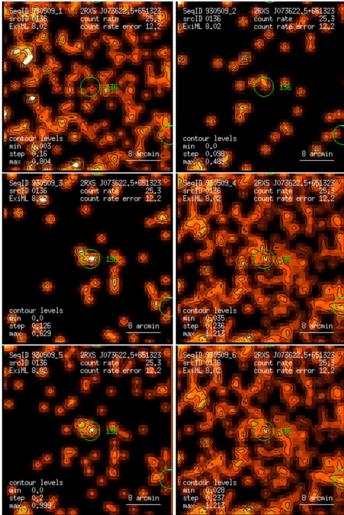
Figure 136: RASS 930509: detection 0136: band rate images, Gaussian filter: (1) PSPC channels 11 – 41, (2) 52 – 90, (3) 91 – 201, (4) 11 – 235, (5) 52 – 201, (6) 11 – 201. Broad band rates in counts/ks. Band rate contour levels in counts/ks/arcmin 2 .
