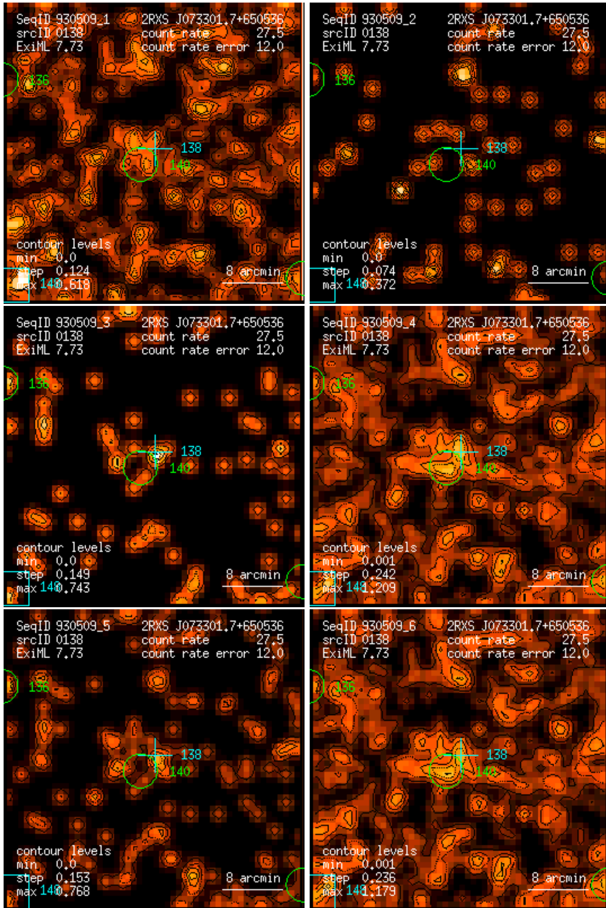
Figure 138: RASS 930509: detection 0138: band rate images, Gaussian filter: (1) PSPC channels 11 – 41, (2) 52 – 90, (3) 91 – 201, (4) 11 – 235, (5) 52 – 201, (6) 11 – 201. Broad band rates in counts/ks. Band rate contour levels in counts/ks/arcmin 2 .
