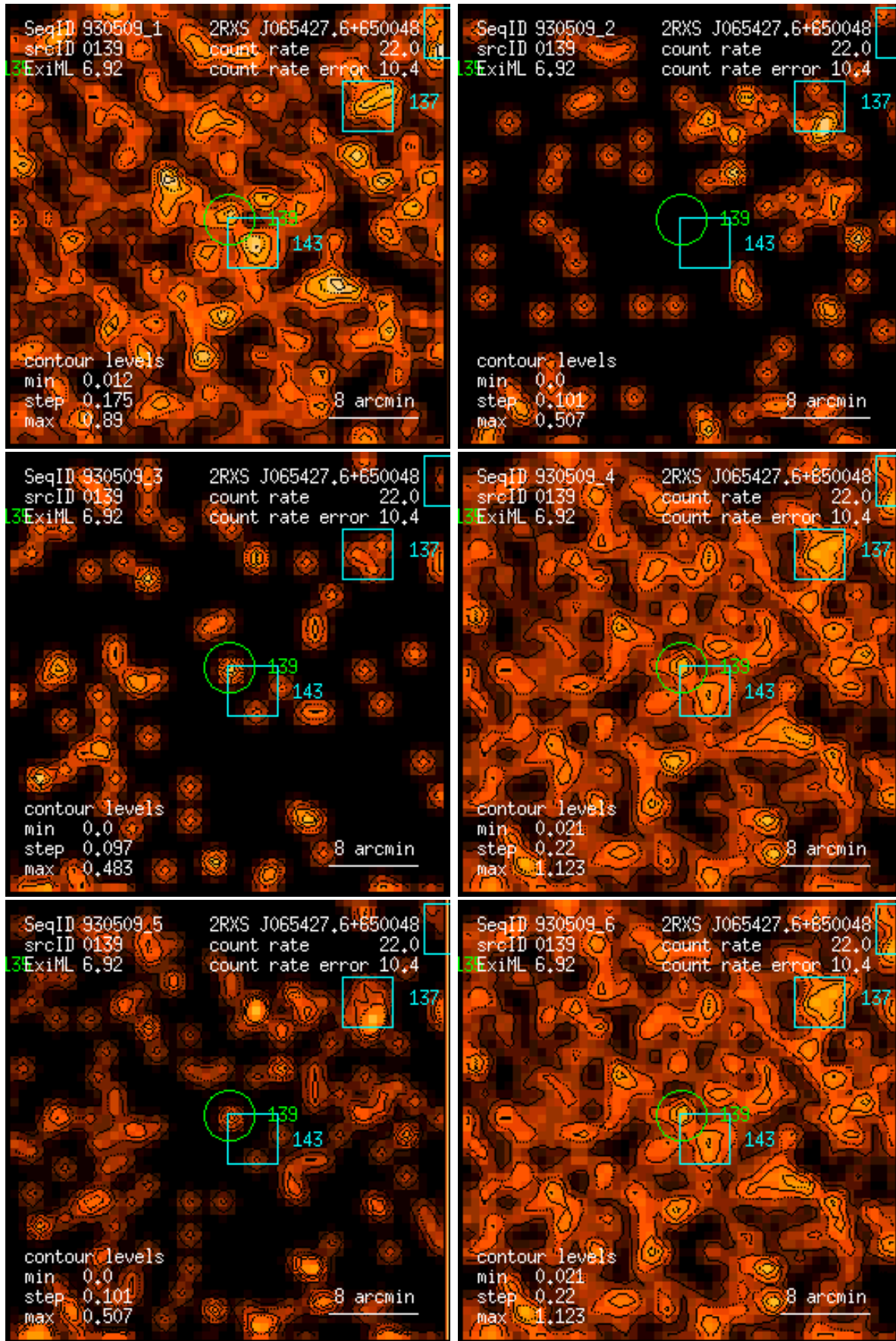
Figure 139: RASS 930509: detection 0139: band rate images, Gaussian filter: (1) PSPC channels 11 – 41, (2) 52 – 90, (3) 91 – 201, (4) 11 – 235, (5) 52 – 201, (6) 11 – 201. Broad band rates in counts/ks. Band rate contour levels in counts/ks/arcmin 2 .
