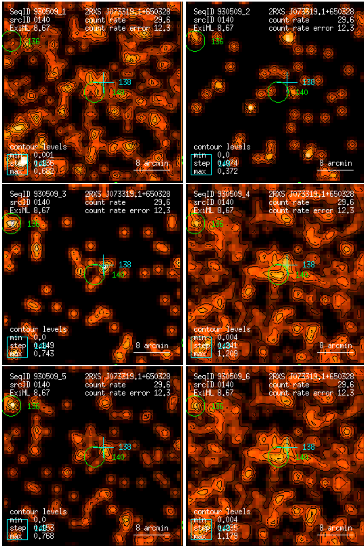
Figure 140: RASS 930509: detection 0140: band rate images, Gaussian filter: (1) PSPC channels 11 – 41, (2) 52 – 90, (3) 91 – 201, (4) 11 – 235, (5) 52 – 201, (6) 11 – 201. Broad band rates in counts/ks. Band rate contour levels in counts/ks/arcmin 2 .
