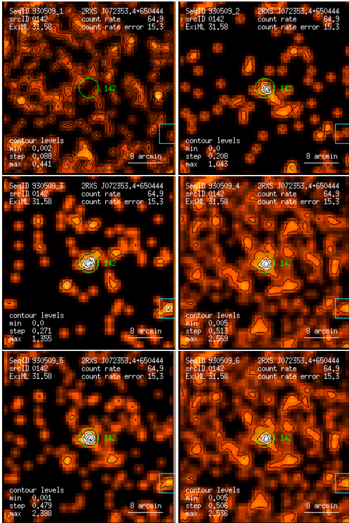
Figure 142: RASS 930509: detection 0142: band rate images, Gaussian filter: (1) PSPC channels 11 – 41, (2) 52 – 90, (3) 91 – 201, (4) 11 – 235, (5) 52 – 201, (6) 11 – 201. Broad band rates in counts/ks. Band rate contour levels in counts/ks/arcmin 2 .
