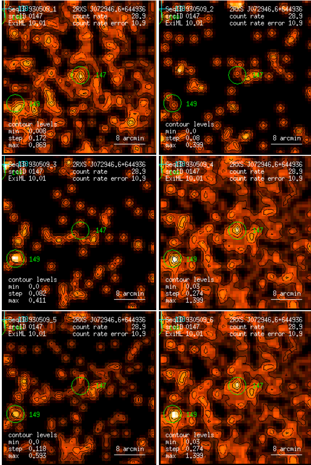
Figure 147: RASS 930509: detection 0147: band rate images, Gaussian filter: (1) PSPC channels 11 – 41, (2) 52 – 90, (3) 91 – 201, (4) 11 – 235, (5) 52 – 201, (6) 11 – 201. Broad band rates in counts/ks. Band rate contour levels in counts/ks/arcmin 2 .
