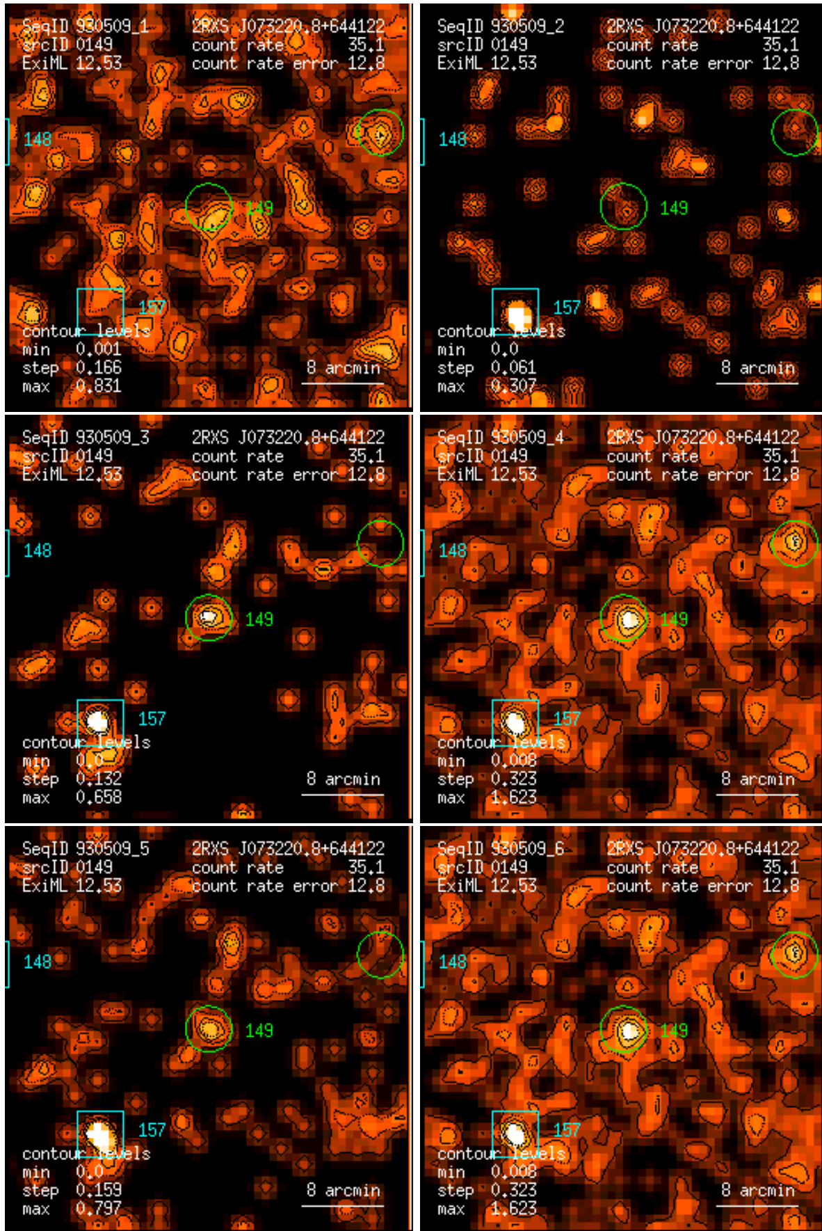
Figure 149: RASS 930509: detection 0149: band rate images, Gaussian filter: (1) PSPC channels 11 – 41, (2) 52 – 90, (3) 91 – 201, (4) 11 – 235, (5) 52 – 201, (6) 11 – 201. Broad band rates in counts/ks. Band rate contour levels in counts/ks/arcmin 2 .
