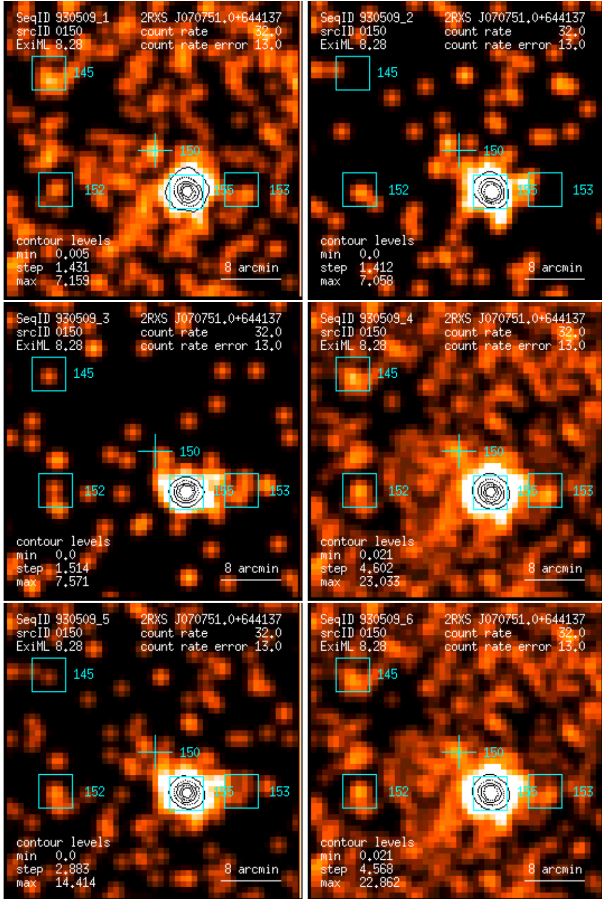
Figure 150: RASS 930509: detection 0150: band rate images, Gaussian filter: (1) PSPC channels 11 – 41, (2) 52 – 90, (3) 91 – 201, (4) 11 – 235, (5) 52 – 201, (6) 11 – 201. Broad band rates in counts/ks. Band rate contour levels in counts/ks/arcmin 2 .
