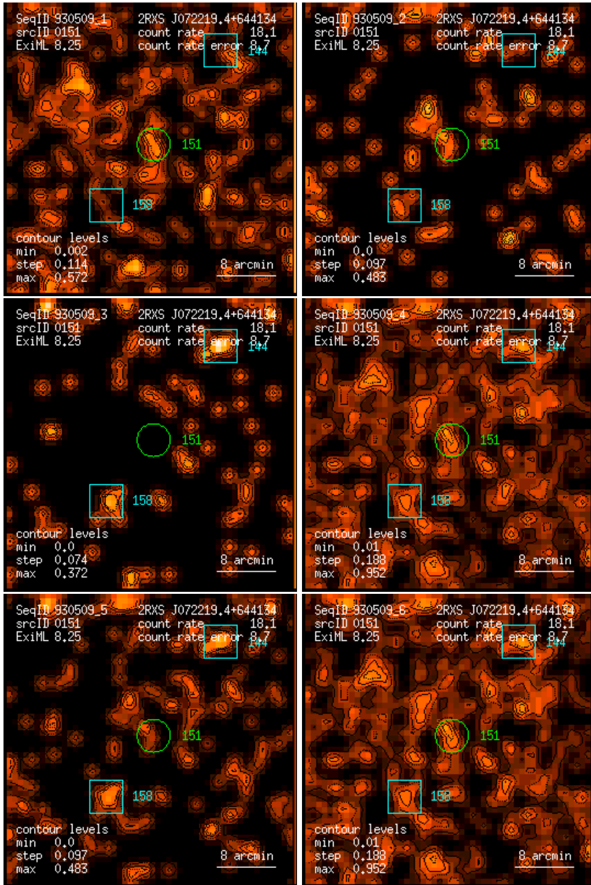
Figure 151: RASS 930509: detection 0151: band rate images, Gaussian filter: (1) PSPC channels 11 – 41, (2) 52 – 90, (3) 91 – 201, (4) 11 – 235, (5) 52 – 201, (6) 11 – 201. Broad band rates in counts/ks. Band rate contour levels in counts/ks/arcmin 2 .
