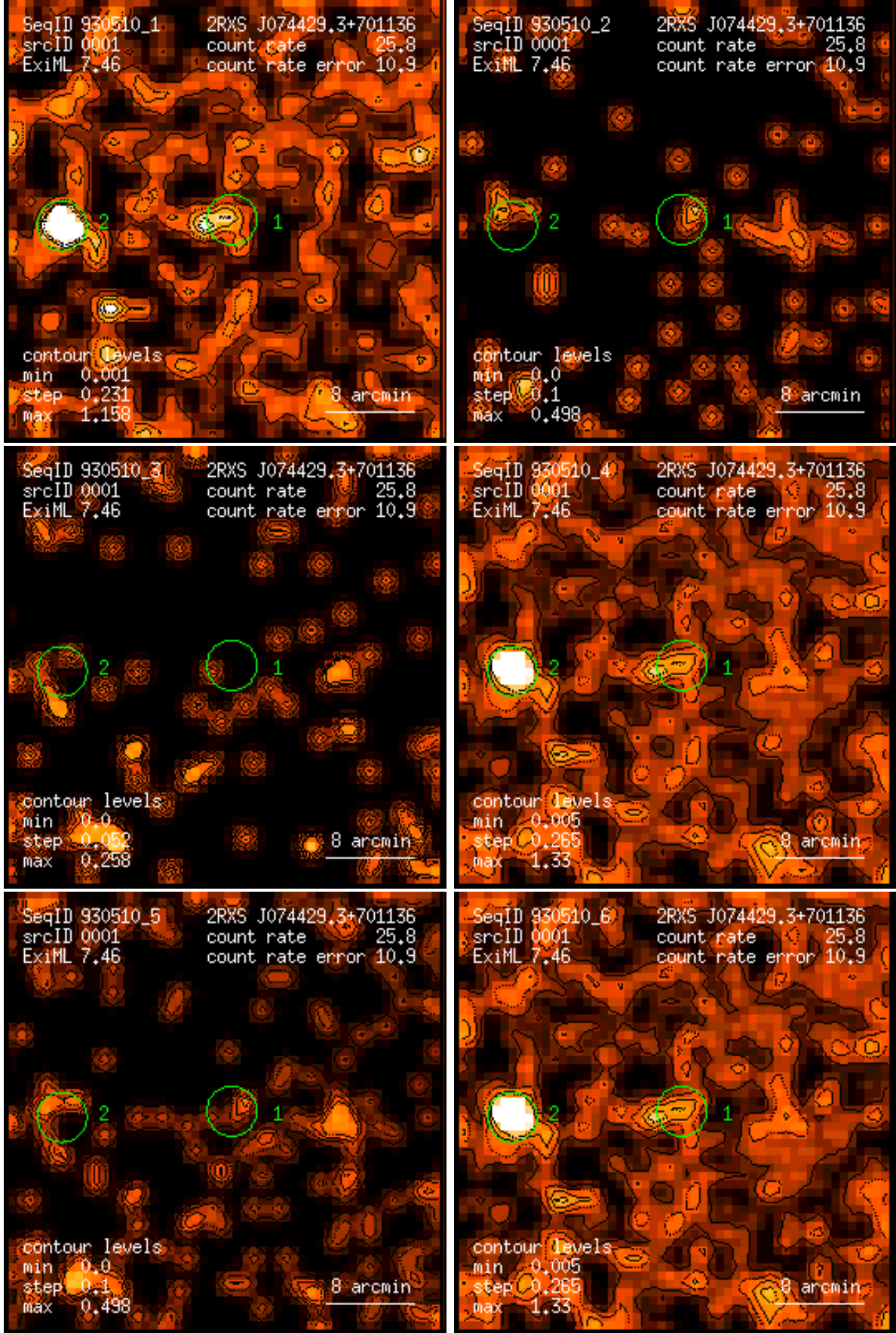
Figure 1: RASS 930510: detection 0001: band rate images, Gaussian filter: (1) PSPC channels 11 – 41, (2) 52 – 90, (3) 91 – 201, (4) 11 – 235, (5) 52 – 201, (6) 11 – 201. Broad band rates in counts/ks. Band rate contour levels in counts/ks/arcmin 2 .
