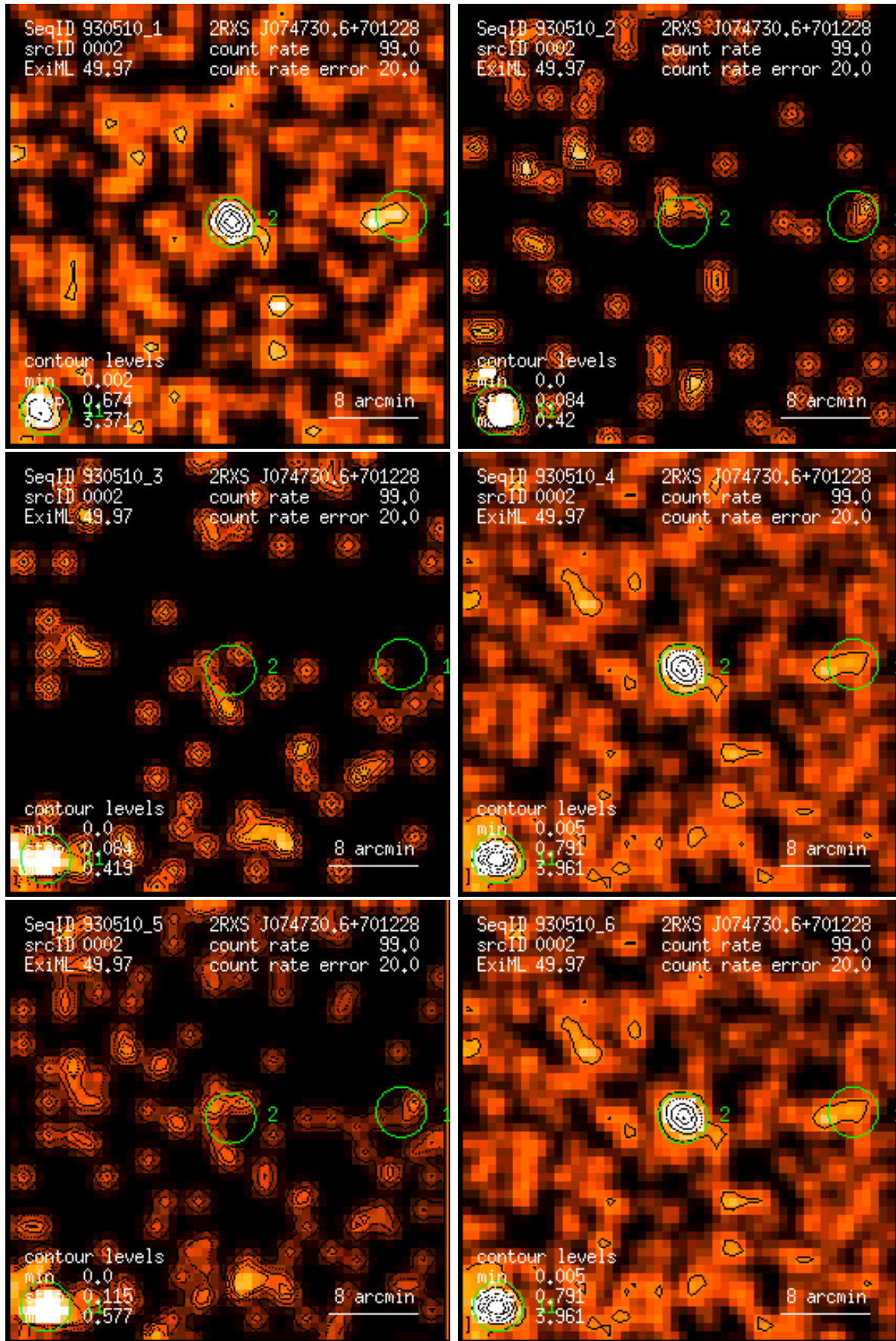
Figure 2: RASS 930510: detection 0002: band rate images, Gaussian filter: (1) PSPC channels 11 – 41, (2) 52 – 90, (3) 91 – 201, (4) 11 – 235, (5) 52 – 201, (6) 11 – 201. Broad band rates in counts/ks. Band rate contour levels in counts/ks/arcmin 2 .
