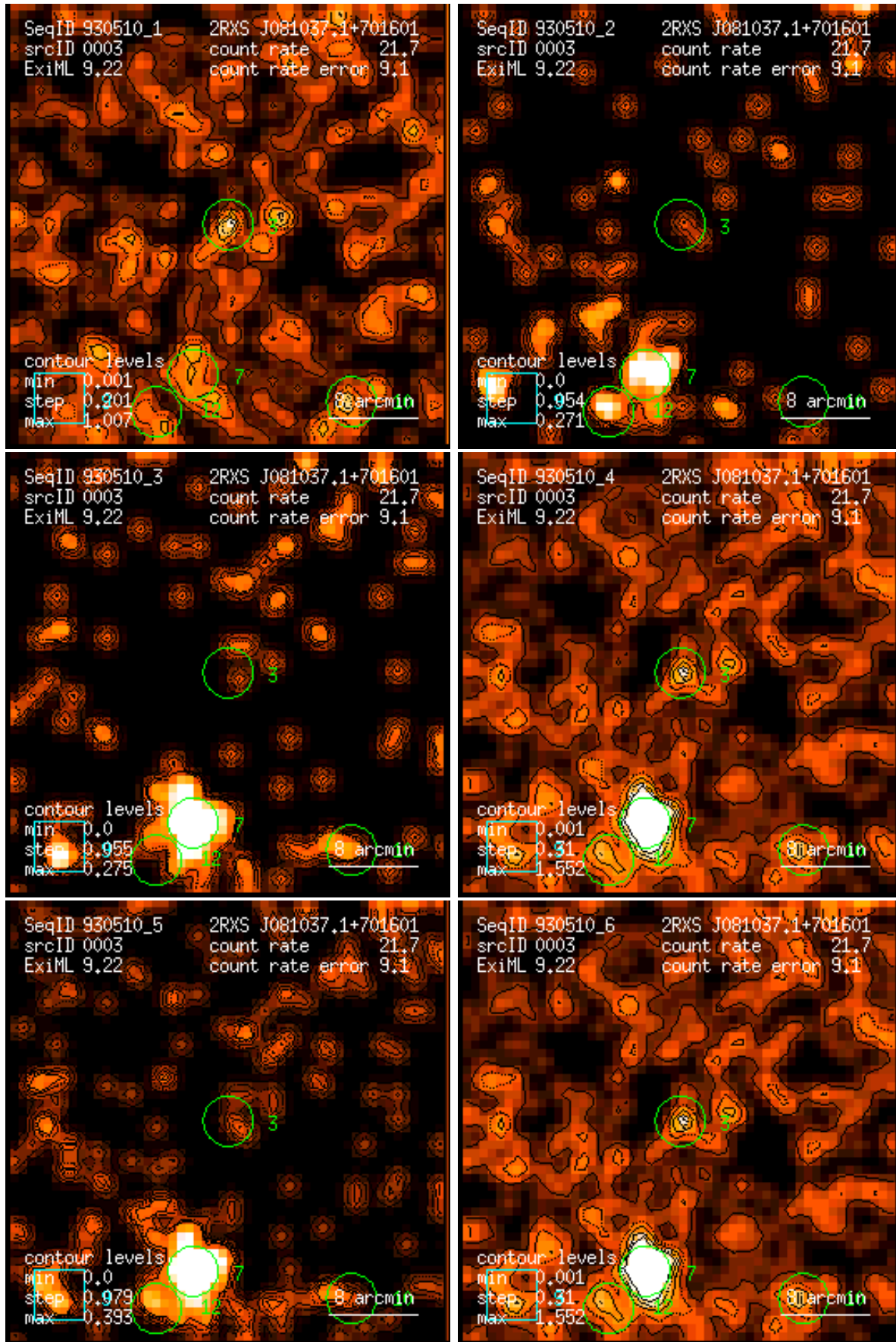
Figure 3: RASS 930510: detection 0003: band rate images, Gaussian filter: (1) PSPC channels 11 – 41, (2) 52 – 90, (3) 91 – 201, (4) 11 – 235, (5) 52 – 201, (6) 11 – 201. Broad band rates in counts/ks. Band rate contour levels in counts/ks/arcmin 2 .
