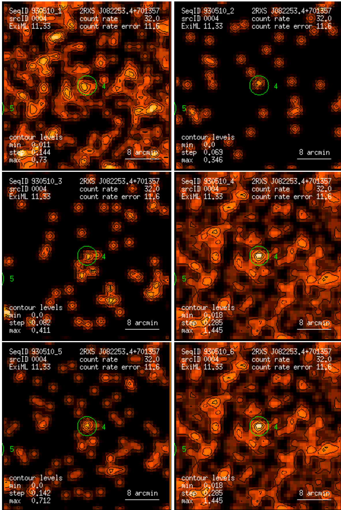
Figure 4: RASS 930510: detection 0004: band rate images, Gaussian filter: (1) PSPC channels 11 – 41, (2) 52 – 90, (3) 91 – 201, (4) 11 – 235, (5) 52 – 201, (6) 11 – 201. Broad band rates in counts/ks. Band rate contour levels in counts/ks/arcmin 2 .
