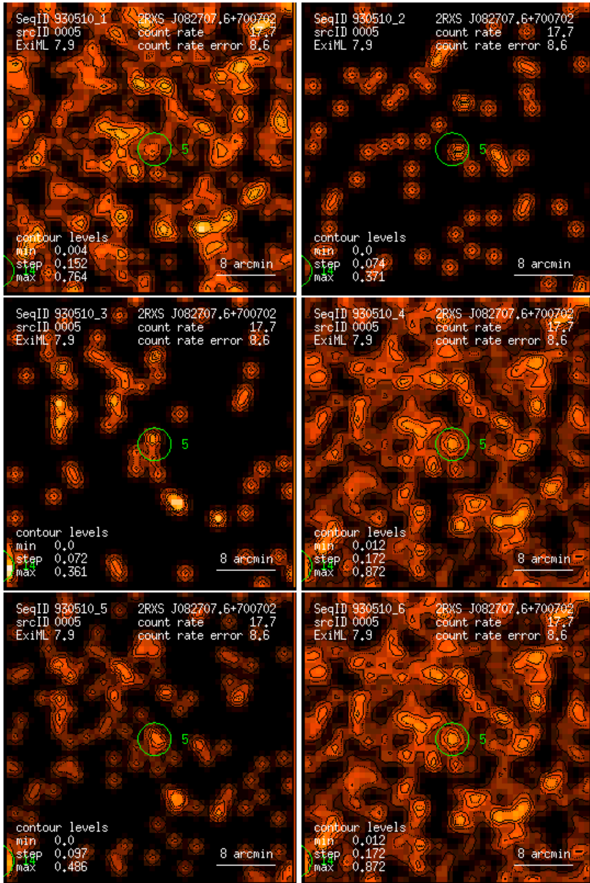
Figure 5: RASS 930510: detection 0005: band rate images, Gaussian filter: (1) PSPC channels 11 – 41, (2) 52 – 90, (3) 91 – 201, (4) 11 – 235, (5) 52 – 201, (6) 11 – 201. Broad band rates in counts/ks. Band rate contour levels in counts/ks/arcmin 2 .
