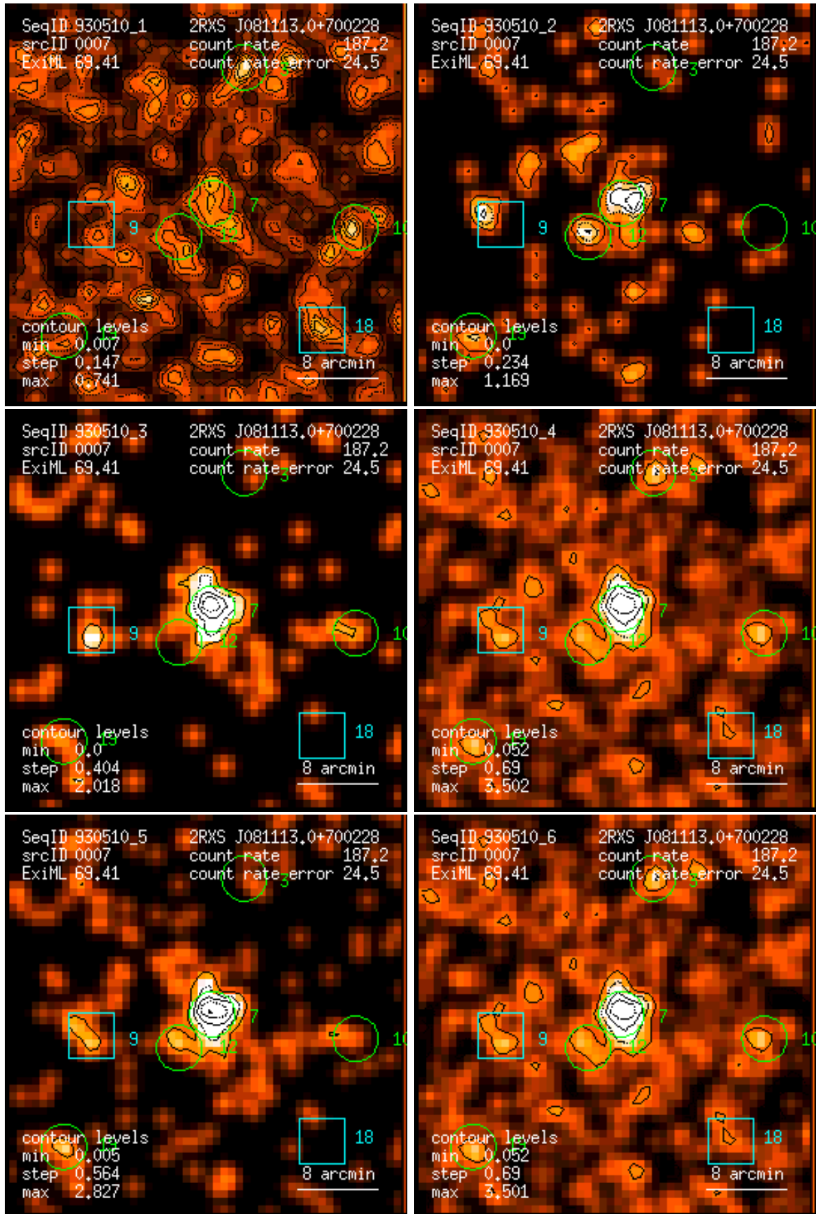
Figure 7: RASS 930510: detection 0007: band rate images, Gaussian filter: (1) PSPC channels 11 – 41, (2) 52 – 90, (3) 91 – 201, (4) 11 – 235, (5) 52 – 201, (6) 11 – 201. Broad band rates in counts/ks. Band rate contour levels in counts/ks/arcmin 2 .
