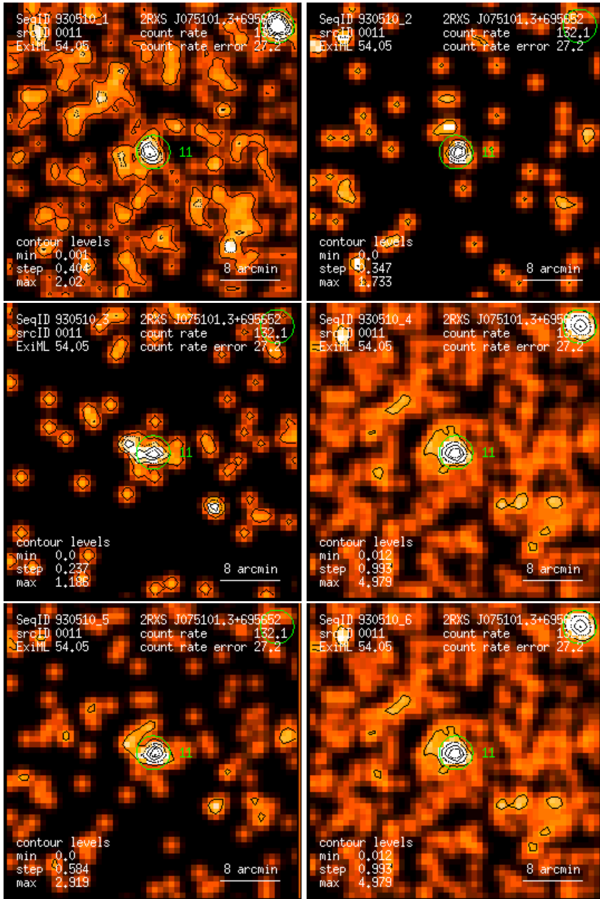
Figure 11: RASS 930510: detection 0011: band rate images, Gaussian filter: (1) PSPC channels 11 – 41, (2) 52 – 90, (3) 91 – 201, (4) 11 – 235, (5) 52 – 201, (6) 11 – 201. Broad band rates in counts/ks. Band rate contour levels in counts/ks/arcmin 2 .
