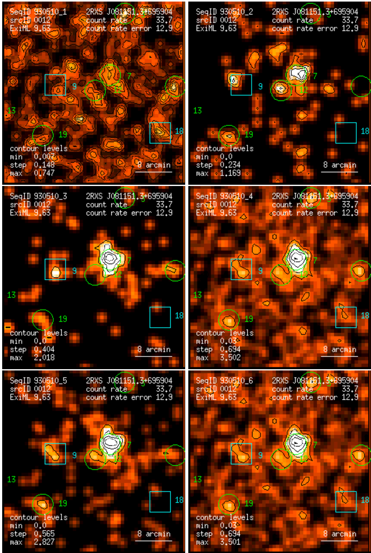
Figure 12: RASS 930510: detection 0012: band rate images, Gaussian filter: (1) PSPC channels 11 – 41, (2) 52 – 90, (3) 91 – 201, (4) 11 – 235, (5) 52 – 201, (6) 11 – 201. Broad band rates in counts/ks. Band rate contour levels in counts/ks/arcmin 2 .
