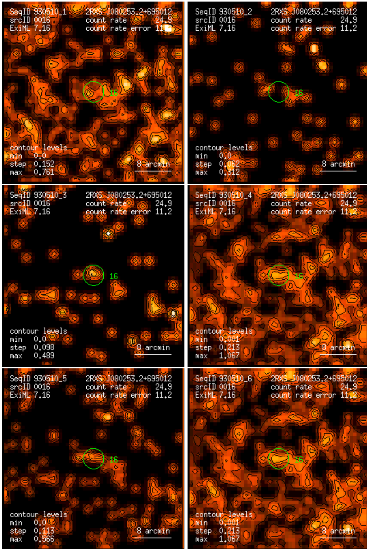
Figure 16: RASS 930510: detection 0016: band rate images, Gaussian filter: (1) PSPC channels 11 – 41, (2) 52 – 90, (3) 91 – 201, (4) 11 – 235, (5) 52 – 201, (6) 11 – 201. Broad band rates in counts/ks. Band rate contour levels in counts/ks/arcmin 2 .
