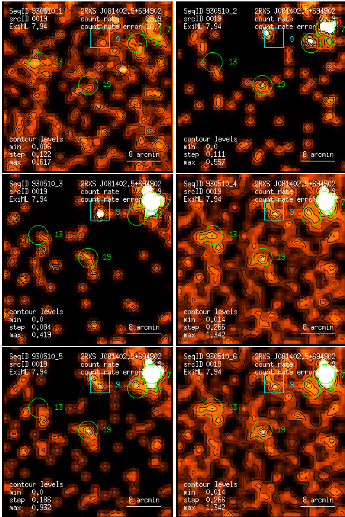
Figure 19: RASS 930510: detection 0019: band rate images, Gaussian filter: (1) PSPC channels 11 – 41, (2) 52 – 90, (3) 91 – 201, (4) 11 – 235, (5) 52 – 201, (6) 11 – 201. Broad band rates in counts/ks. Band rate contour levels in counts/ks/arcmin 2 .
