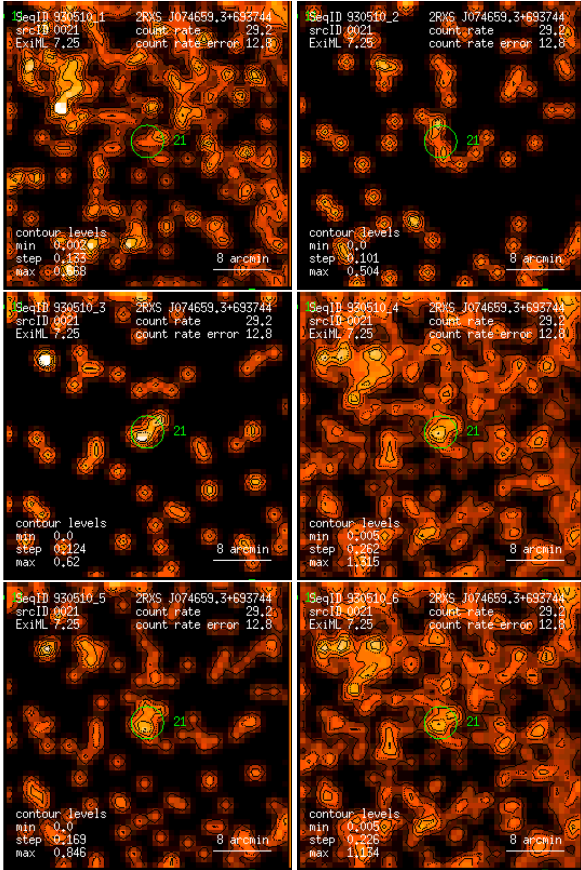
Figure 21: RASS 930510: detection 0021: band rate images, Gaussian filter: (1) PSPC channels 11 – 41, (2) 52 – 90, (3) 91 – 201, (4) 11 – 235, (5) 52 – 201, (6) 11 – 201. Broad band rates in counts/ks. Band rate contour levels in counts/ks/arcmin 2 .
